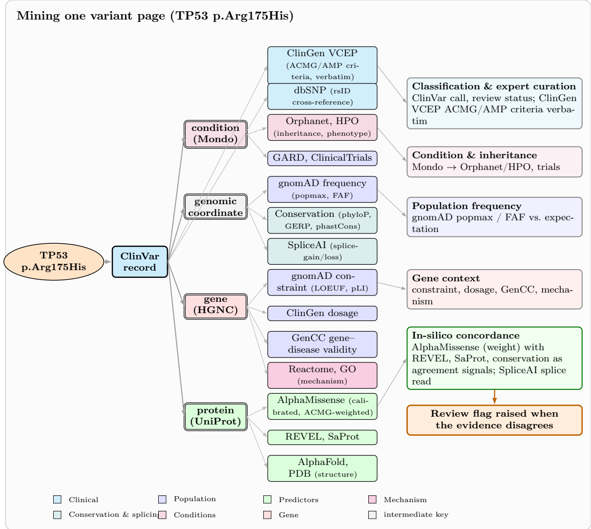
Figure 2: Mining one variant page. Each leaf is a BioBTree dataset the page queries, fanned from the resolved ClinVar anchor (here the TP53 variant p.Arg175His) through the intermediate keys the variant resolves to: the condition (Mondo, and thence Orphanet and HPO for inheritance and phenotype, and patient resources and trials); the genomic coordinate (gnomAD population frequency, sequence conservation, and SpliceAI); the gene (gnomAD constraint, ClinGen dosage, GenCC gene-disease validity, and Reactome mechanism pathways); and the protein change (AlphaMissense, REVEL, SaProt, and the reviewed structure). The ClinGen expert-panel curation and the dbSNP cross-reference are reached directly from the ClinVar record. The right-hand column shows how those data assemble into the sections of the page. AlphaMissense carries the calibrated ACMG weight, with REVEL, SaProt, and conservation shown as agreement signals rather than additive votes and SpliceAI as a splice read, so the in-silico concordance of Section 2.3 is a descriptive quality-control read, and the variant is flagged for review when the evidence disagrees. Colours group the datasets by evidence type, as in Figure 1.
