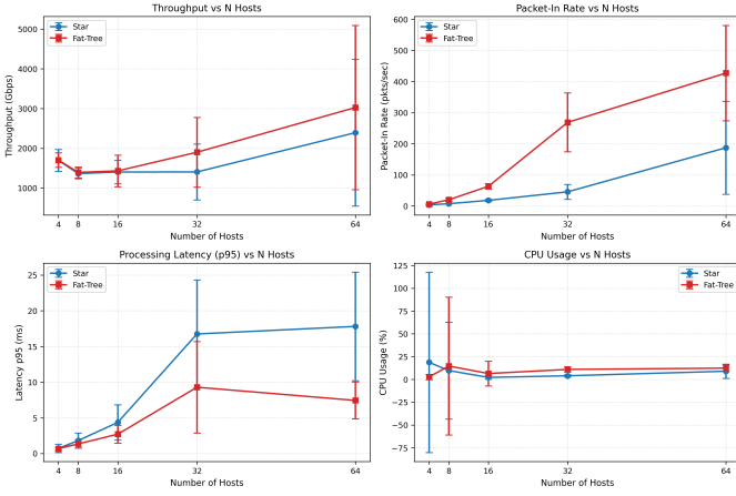
Fig. 5. Scalability: throughput, Packet-In rate, p95 latency, and CPU vs. host count. Star p95 plateaus at \sim 17 ms beyond N=32 ; fat-tree remains lower across all scales.
