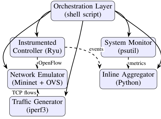
Fig. 1. Testbed architecture. The orchestration layer coordinates all components; the aggregator consolidates per-run outputs.
