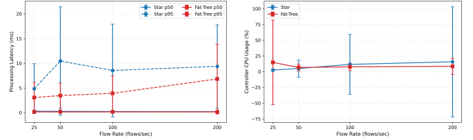
(a) Processing latency (p50 and p95) vs. flow rate
