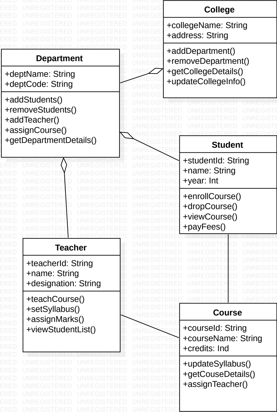
Model1::ClassDiagram1
