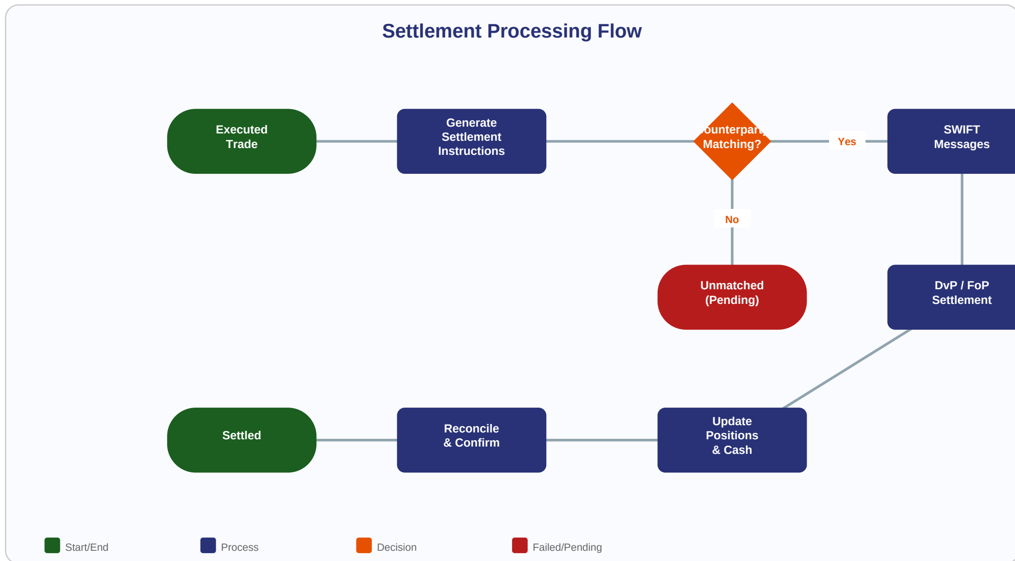
Figure 4: Settlement Processing Flow
