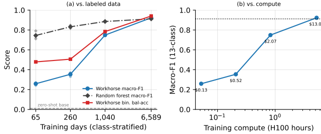
Fig. 3. The data-efficiency curves of the workhorse and the matched random-forest refits: (a) macro-F1 against training-set size, with the workhorse’s binary balanced accuracy; (b) workhorse macro-F1 against training compute (the forest trains in CPU-minutes at every size). Per-seed points shown at N=65 and N=260 . The forest dominates until full data.
