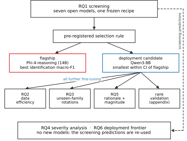
Fig. 1. The dependency structure of the experiments. One screening pass fine-tunes all seven models under the frozen recipe; the pre-registered rule selects the flagship and the deployment candidate from its results; every later fine-tuning run, covering the data-efficiency curve (RQ2), the unseen-family rotations (RQ3), the rationale and magnitude extensions (RQ5), and the rank validation of Appendix A, trains the deployment candidate alone. The severity analysis (RQ4) and the deployment frontier (RQ6) fit no new models and re-use the screening predictions.
