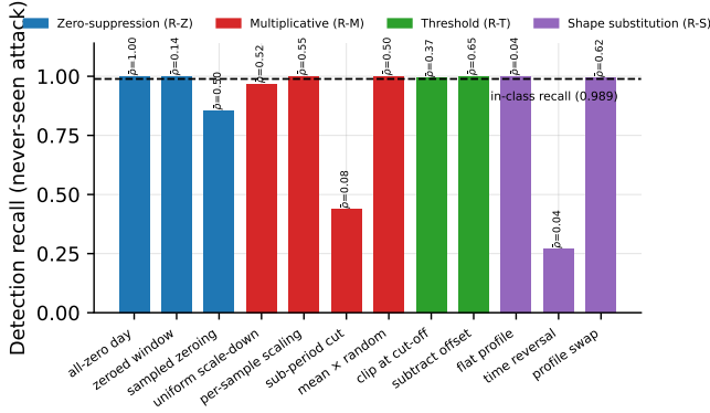
Fig. 6. Detection recall per never-seen attack, grouped by held-out rotation and annotated with the mean energy-removal proxy \bar{\rho} . The horizontal line is the in-class recall of the deployment candidate (0.989).
