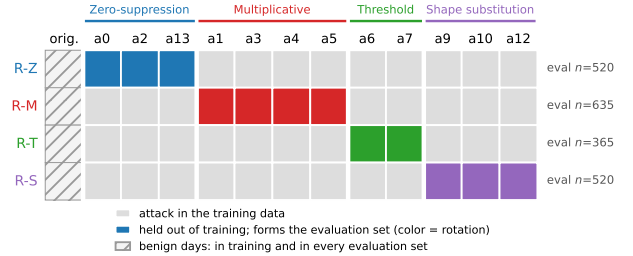
Fig. 5. The train/evaluation design of the four rotations. Each row retrains the deployment candidate with one attack family removed: gray cells mark the attacks left in the training data, colored cells the held-out family that forms the manipulated half of that rotation’s evaluation set, and the hatched column the benign days, which stay in training and in every evaluation set. The random forest is retrained on the identical reduced sets.
