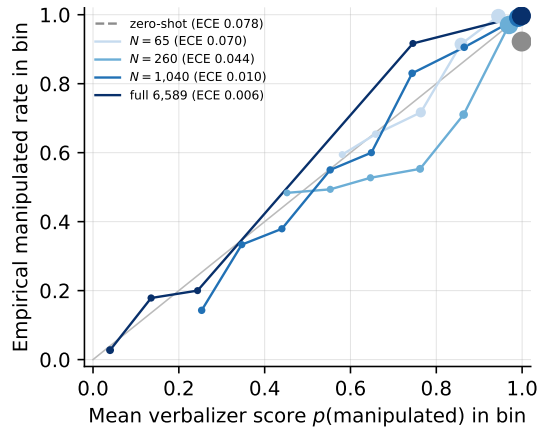
Fig. 10. Reliability of the verbalizer score across training stages (ten equal-width bins on the evaluation slice; multi-seed stages show the seed-mean curve). Bins holding at least ten days are drawn, with marker area tracking bin support; the expected calibration error in the legend is computed over all bins, support-weighted. Discrimination precedes calibration: the AUC is high from the start while the calibration gap closes only with the full training data.
