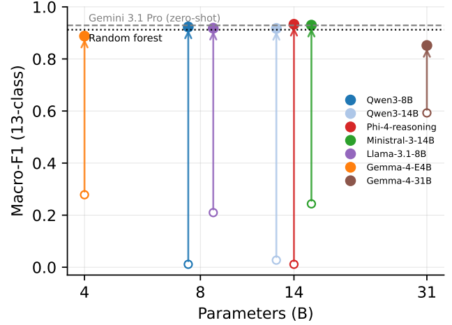
Fig. 2. Macro-F1 against parameter count before and after fine-tuning. Each arrow joins a model’s zero-shot score to its fine-tuned score; same-size models are dodged horizontally for legibility. The dashed band is the zero-shot Gemini 3.1 Pro score and the dotted band the random forest baseline.
