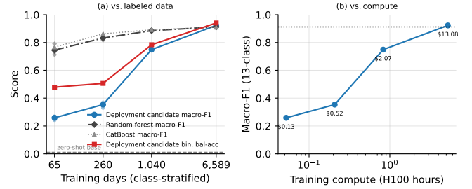
Fig. 4. The data-efficiency curves of the deployment candidate and the classical baselines trained on the identical subsets: (a) macro-F1 against training-set size, with the deployment candidate’s binary balanced accuracy; (b) deployment candidate macro-F1 against training compute (the classical models train in CPU-minutes at every size). Per-seed points shown at N=65 and N=260 ; XGBoost (slightly below the forest throughout) is omitted for legibility and tabulated in Appendix D. Every classical variant dominates until full data.
