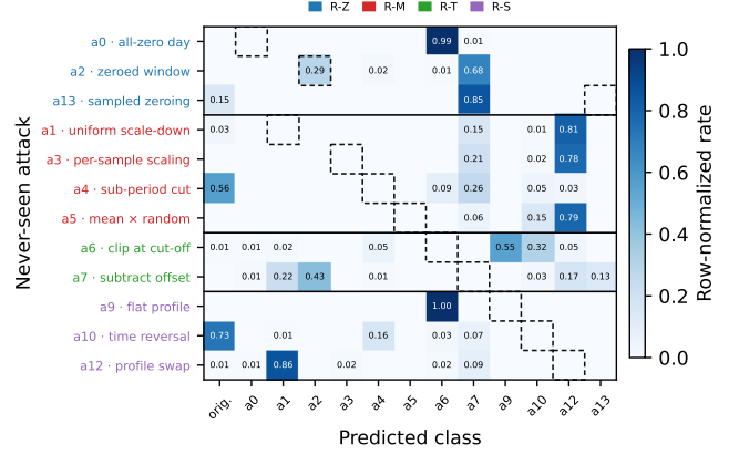
Fig. 7. Identification confusion for the never-seen attacks. Each row is a held-out attack, grouped and colored by rotation; each column is a predicted class, row-normalized over that attack’s evaluation days. The dashed cell in each row marks the correct name. Prediction mass concentrates on trained attacks of similar mechanism, and the original column collects the detection misses of Table VII.
