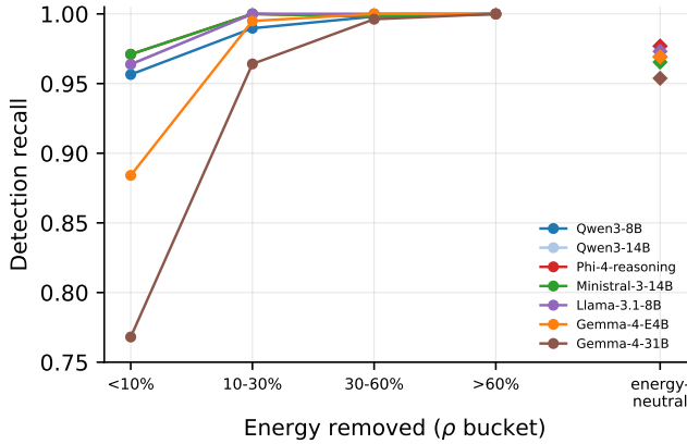
Fig. 8. Detection recall against theft severity for the screened models, with the energy-neutral pair (total energy unchanged, profile reshaped) as detached markers. Every model saturates above 60% energy removal; the differences live below 10%.
