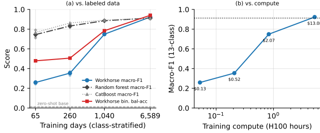
Fig. 3. The data-efficiency curves of the workhorse and the matched classical refits: (a) macro-F1 against training-set size, with the workhorse’s binary balanced accuracy; (b) workhorse macro-F1 against training compute (the classical models train in CPU-minutes at every size). Per-seed points shown at N=65 and N=260 ; XGBoost (slightly below the forest throughout) is omitted for legibility and tabulated in Appendix D. Every classical variant dominates until full data.
