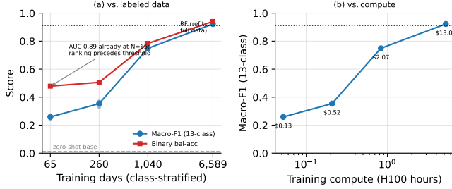
Fig. 3. The data-efficiency curve of the workhorse: (a) macro-F1 and binary balanced accuracy against training-set size; (b) macro-F1 against training compute. Per-seed points shown at N=65 and N=260 ; reference lines are the refit random forest (full data) and the zero-shot base.
