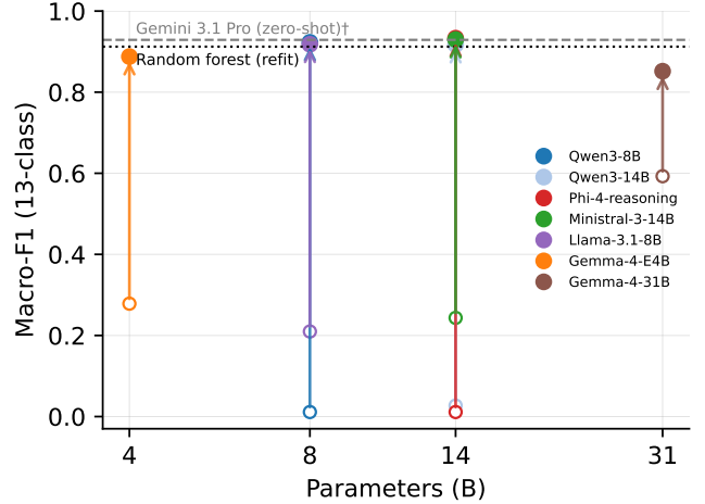
Fig. 1. Macro-F1 against parameter count before and after fine-tuning. Each arrow joins a model’s zero-shot score to its fine-tuned score; the dashed band is the frozen Gemini 3.1 Pro reference and the dotted band the refit random forest.
