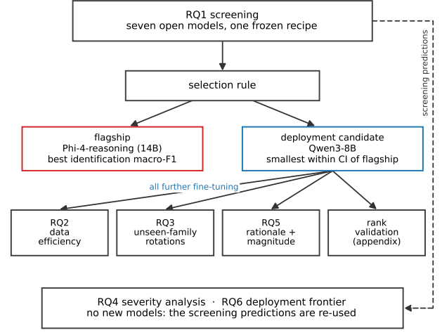
Fig. 1. The dependency structure of the experiments. The screening fine-tunes all seven models under the frozen recipe; the selection rule picks the flagship and the deployment candidate from its results; every later fine-tuning run, covering the data-efficiency curve (RQ2), the unseen-family rotations (RQ3), the rationale and magnitude extensions (RQ5), and the rank validation of Appendix A, trains the deployment candidate alone. The severity analysis (RQ4) and the deployment frontier (RQ6) fit no new models and re-use the screening predictions.
