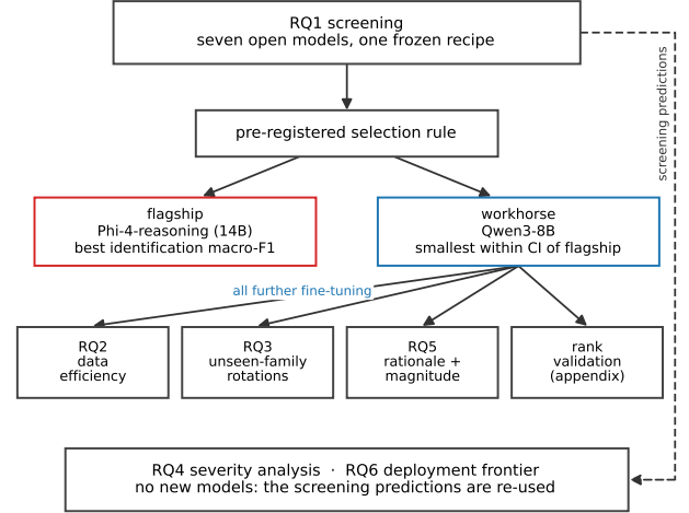
Fig. 1. The dependency structure of the experiments. One screening pass fine-tunes all seven models under the frozen recipe; the pre-registered rule selects the flagship and the workhorse from its results; every later fine-tuning run, covering the data-efficiency curve (RQ2), the unseen-family rotations (RQ3), the rationale and magnitude extensions (RQ5), and the rank validation of Appendix A, trains the workhorse alone. The severity analysis (RQ4) and the deployment frontier (RQ6) fit no new models and re-use the screening predictions.
