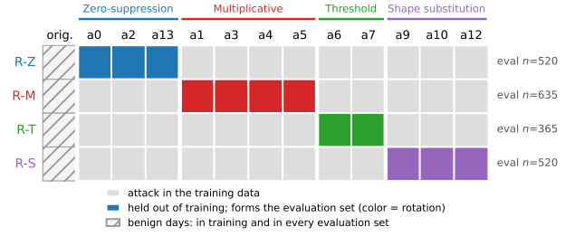
Fig. 5. The train/evaluation design of the four rotations. Each row retrains the workhorse with one attack family removed: gray cells mark the attacks left in the training data, colored cells the held-out family that forms the manipulated half of that rotation’s evaluation set, and the hatched column the benign days, which stay in training and in every evaluation set. The random forest is retrained on the identical reduced sets.
