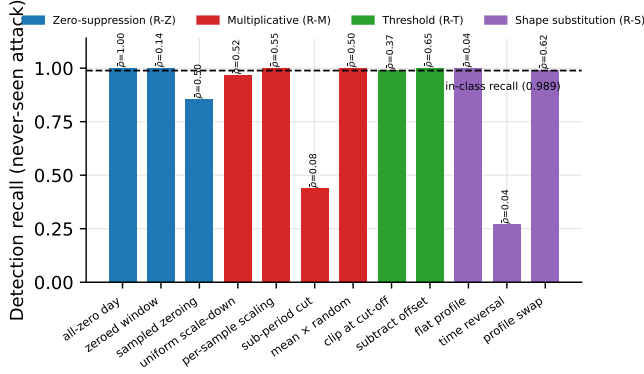
Fig. 6. Detection recall per never-seen attack, grouped by held-out rotation and annotated with the mean energy-removal proxy \bar{\rho} . The horizontal line is the in-class recall of the workhorse (0.989).
