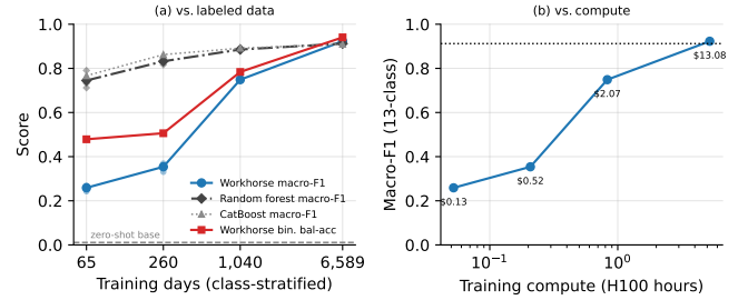
Fig. 4. The data-efficiency curves of the workhorse and the classical baselines trained on the identical subsets: (a) macro-F1 against training-set size, with the workhorse’s binary balanced accuracy; (b) workhorse macro-F1 against training compute (the classical models train in CPU-minutes at every size). Per-seed points shown at N=65 and N=260 ; XGBoost (slightly below the forest throughout) is omitted for legibility and tabulated in Appendix D. Every classical variant dominates until full data.
