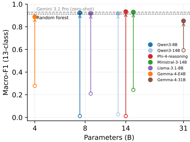
Fig. 2. Macro-F1 against parameter count before and after fine-tuning. Each arrow joins a model’s zero-shot score to its fine-tuned score; same-size models are dodged horizontally for legibility. The dashed band is the zero-shot Gemini 3.1 Pro score and the dotted band the random forest baseline.
