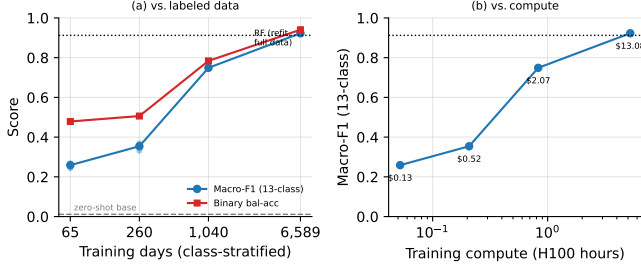
Fig. 3. The data-efficiency curve of the workhorse: (a) macro-F1 and binary balanced accuracy against training-set size; (b) macro-F1 against training compute. Per-seed points shown at N=65 and N=260 ; reference lines are the refit random forest (full data) and the zero-shot base.
