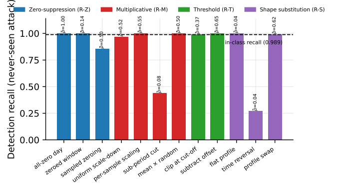
Fig. 4. Detection recall per never-seen attack, grouped by held-out rotation and annotated with the mean energy-removal proxy \bar{p} . The horizontal line is the in-class recall of the workhorse (0.989).
