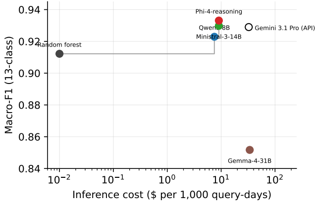
Fig. 7. The cost–performance frontier: macro-F1 against inference cost per 1,000 query-days (log scale). The step line traces the Pareto front; the open marker is the zero-shot API point. The cascade operating point is reported in the frontier table.
