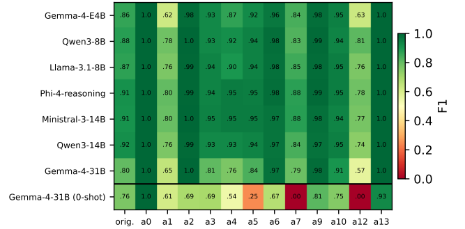
Fig. 2. Per-class F1 for the seven fine-tuned models, ordered by parameter count, with the best zero-shot model (Gemma-4-31B) as the bottom row for contrast. attack1 and attack12 limit every model.
