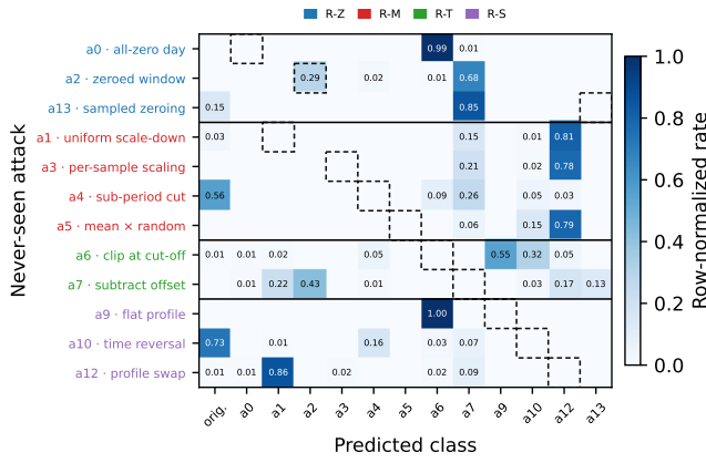
Fig. 5. Identification confusion for the never-seen attacks. Each row is a held-out attack, grouped and colored by rotation; each column is a predicted class, row-normalized over that attack's evaluation days. The dashed cell in each row marks the correct name. Prediction mass concentrates on trained attacks of similar mechanism, and the original column collects the detection misses of Table VII.
