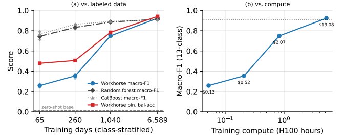
Fig. 3. The data-efficiency curves of the workhorse and the classical baselines trained on the identical subsets: (a) macro-F1 against training-set size, with the workhorse’s binary balanced accuracy; (b) workhorse macro-F1 against training compute (the classical models train in CPU-minutes at every size). Per-seed points shown at N=65 and N=260 ; XGBoost (slightly below the forest throughout) is omitted for legibility and tabulated in Appendix D. Every classical variant dominates until full data.
