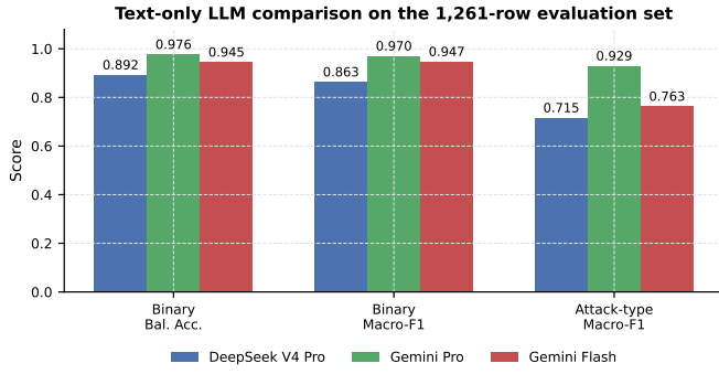
Fig. 3. Comparison of the three completed text-only LLM runs. Gemini Pro is best on binary balanced accuracy, binary macro-F1, and attack-type macro-F1.
