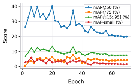
(h) TOOD R50
