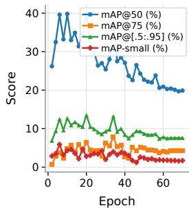
(h) TOOD R50
