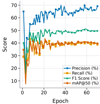
(b) YOLOv10m
