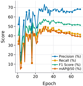
(a) YOLOv9m @1280
