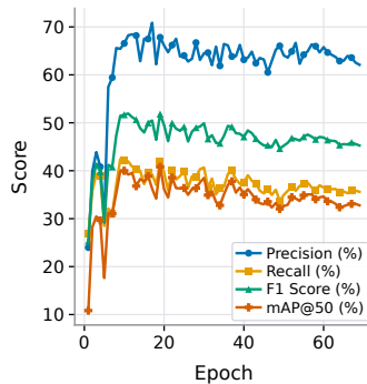
(g) RT-DETR-L
