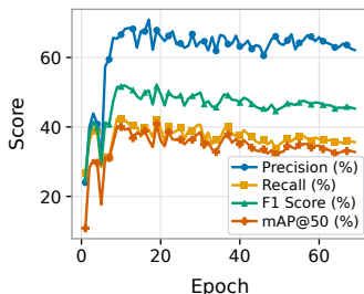
(f) RT-DETR-L
