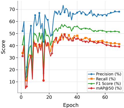
(a) YOLOv9m @1280
