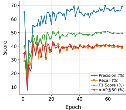
(b) YOLOv10m
