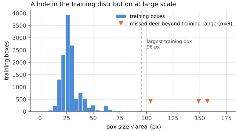
Fig. 10 A hole in the training distribution. The training split contains no box above 96 px. Three missed animals sit at 104, 149 and 157 px, one of them never detected at all. A detector that finds 27 px animals does not miss a 149 px one unless it has never seen one.
