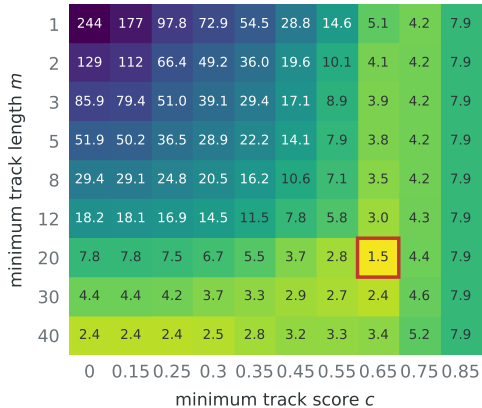
Fit set (19 training videos)
