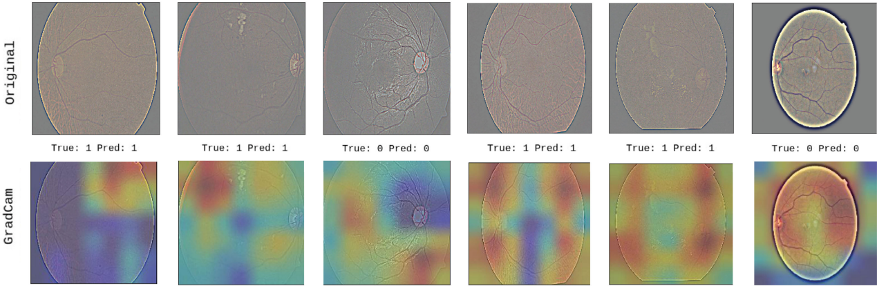
FIGURE 9. Grad-cam results from the test set.
