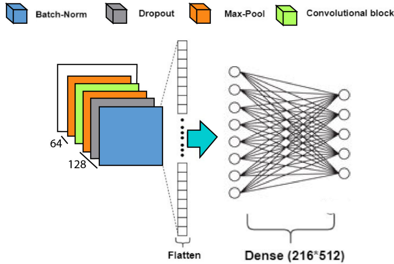
FIGURE 3. Proposed model architecture.
