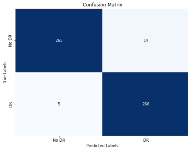
FIGURE 7. Confusion matrix of the proposed model.
