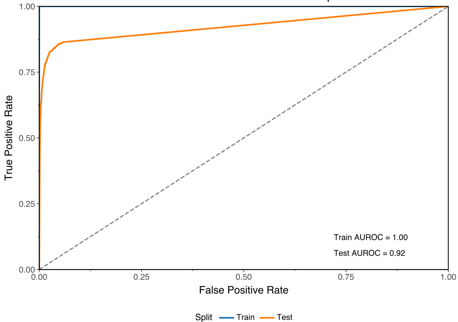
ROC Curves for Train and Test Splits
