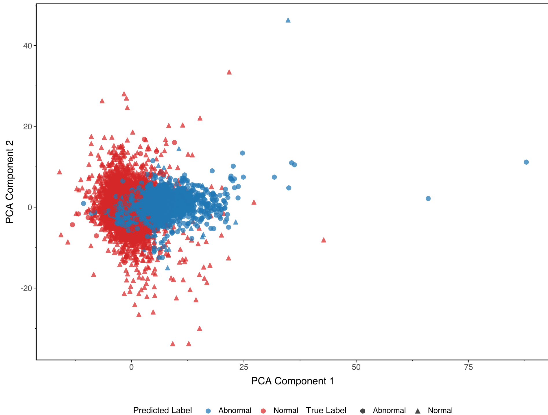
Termite-Inspired Stigmergy Classifier on ECG Beat Embeddings
