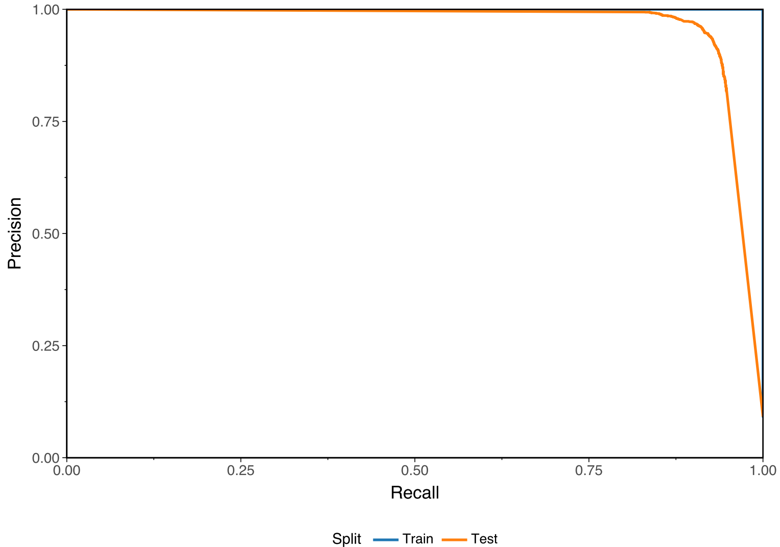
Precision–Recall Curves for the Abnormal Class
