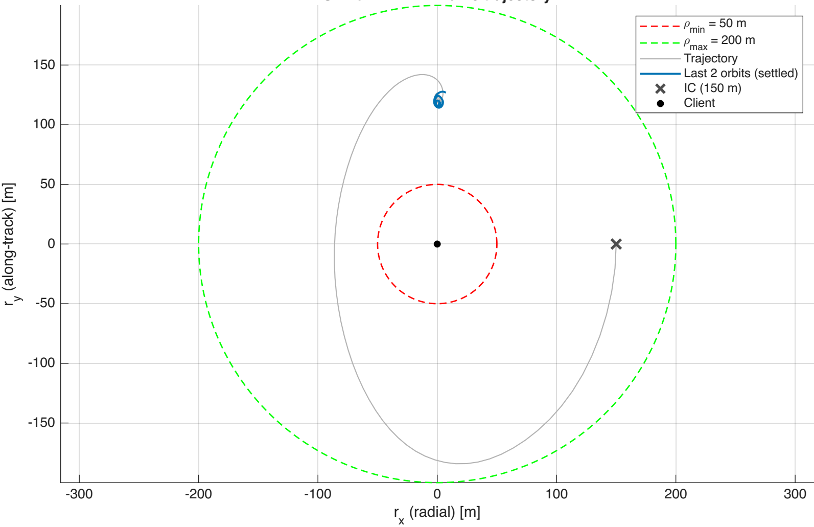
S2 Run 1 — Hill-frame trajectory
