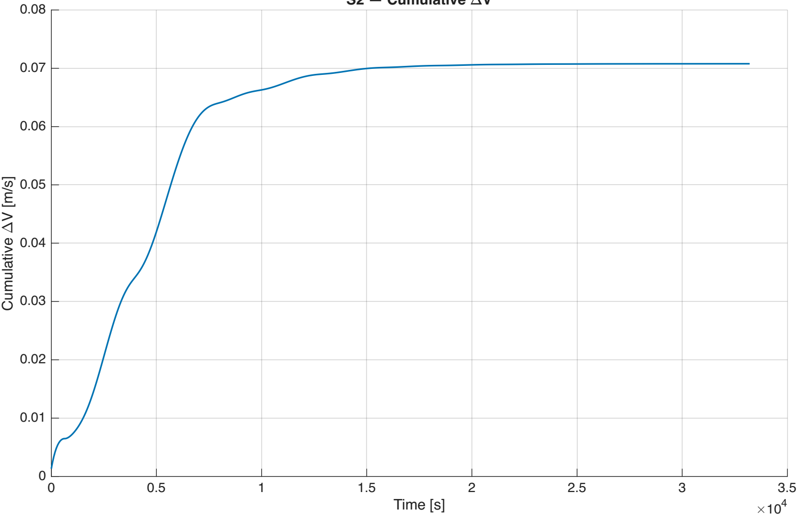
S2 — Cumulative \Delta V
