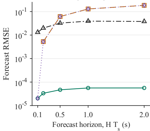
(a) Exact-sine model (Plant B)
