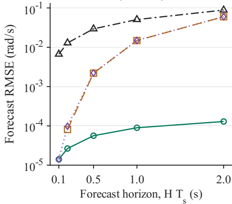
(b) Integrated physical model (Plant C)
