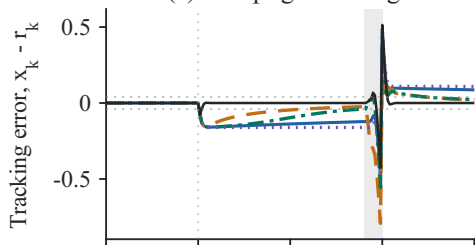
(a) Abrupt gain change
