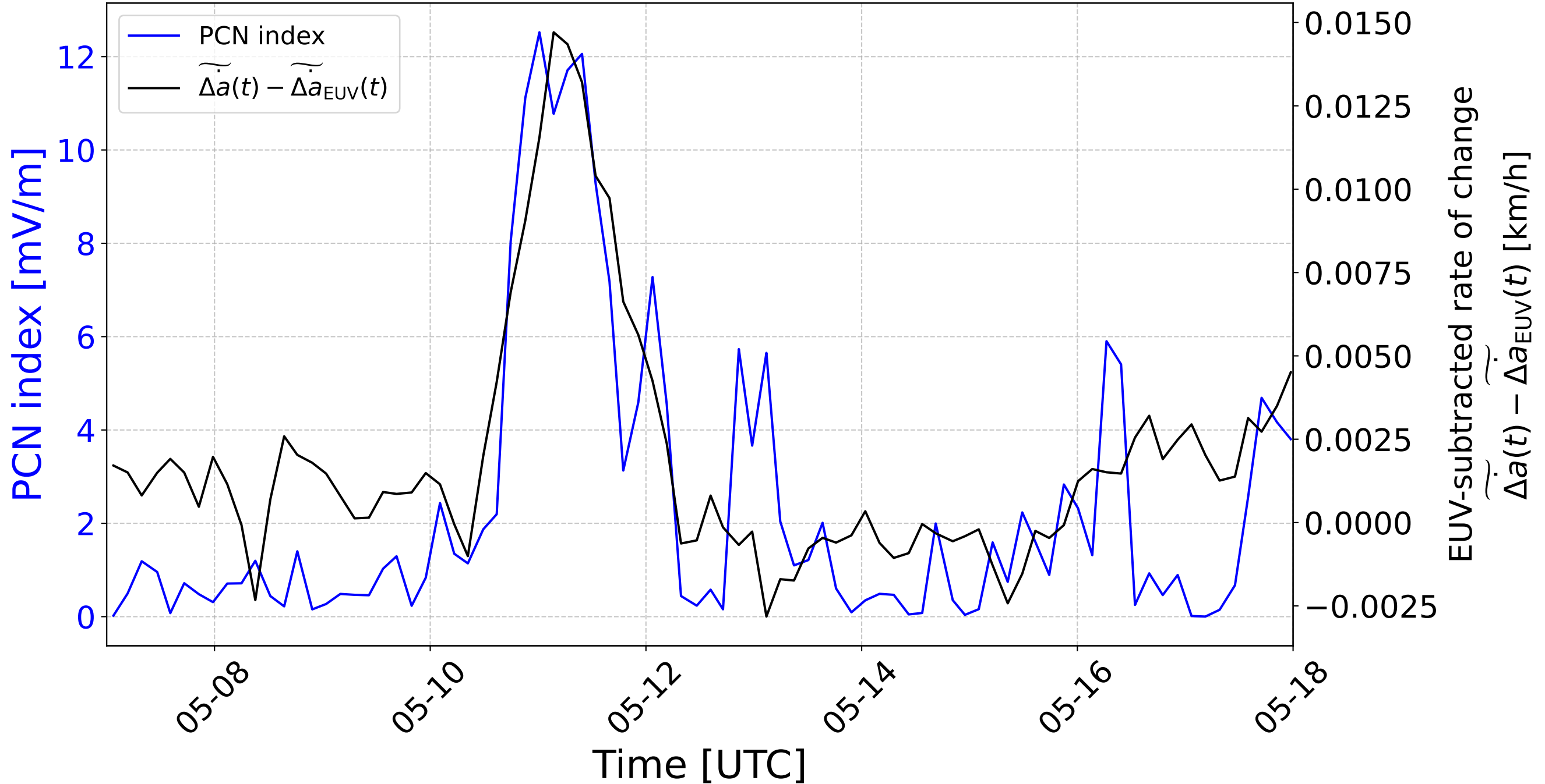
PCN index and EUV-subtracted rate of change for May 2024
