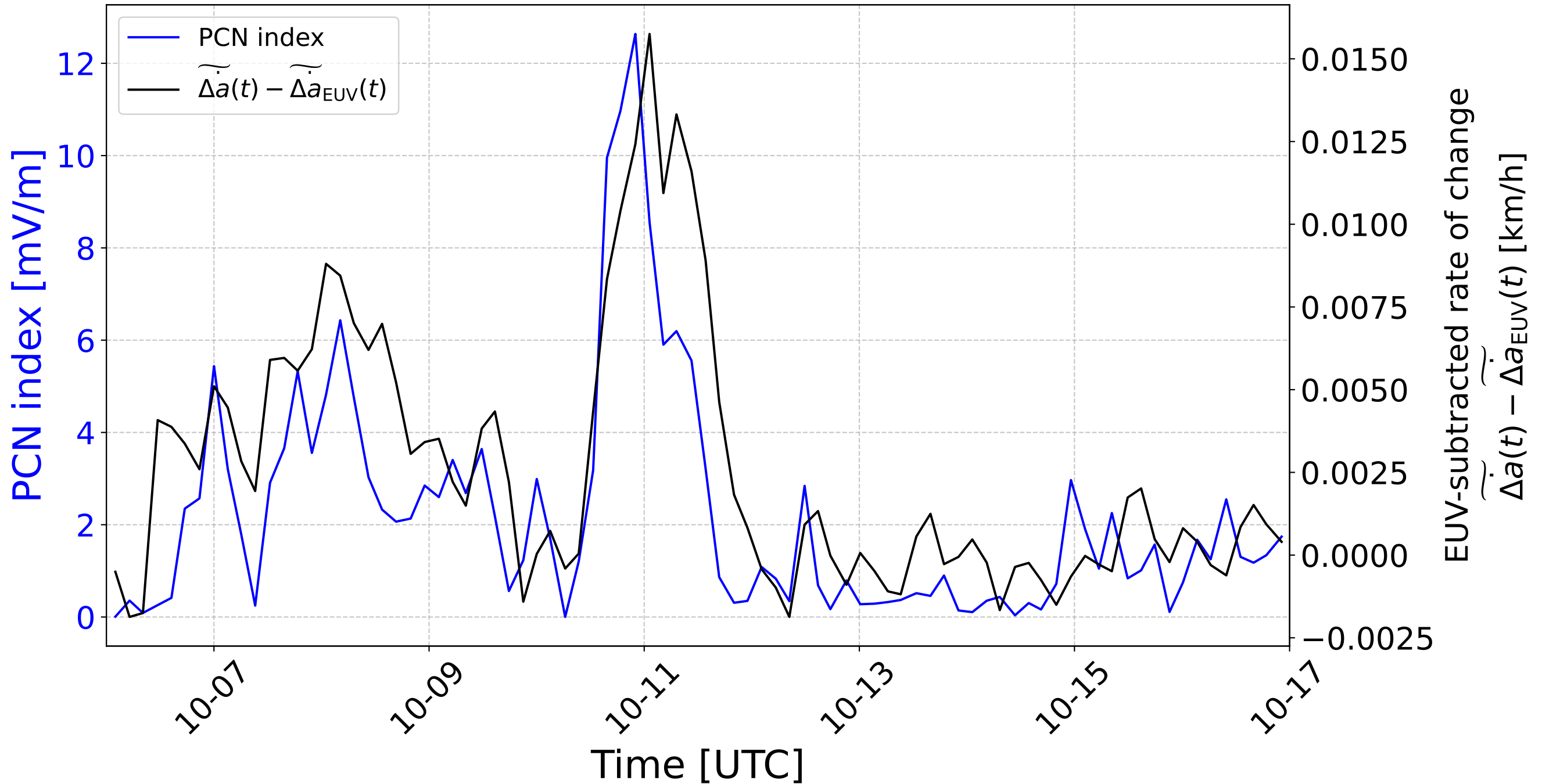
PCN index and EUV-subtracted rate of change for October 2024
