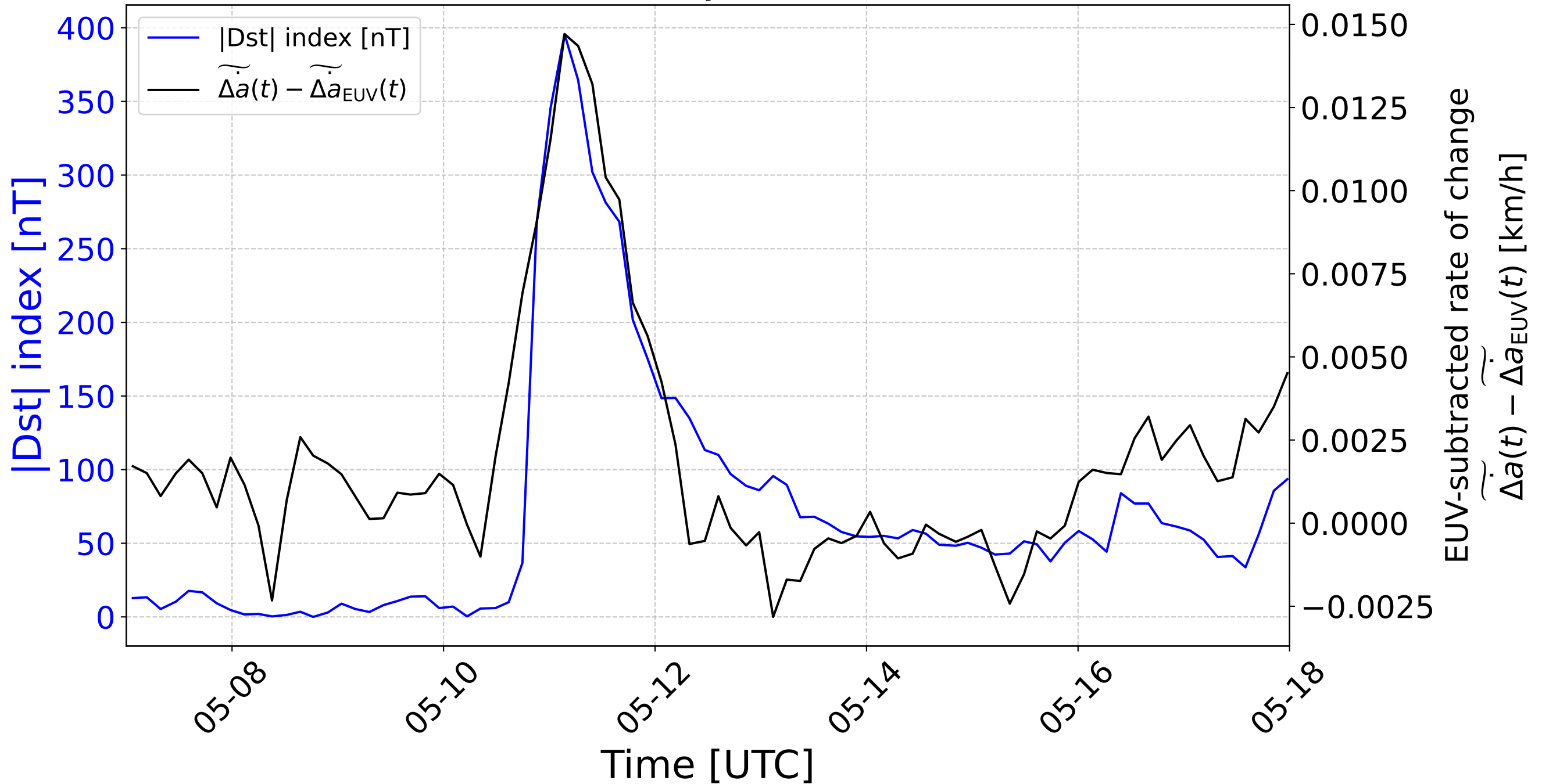
|Dst| index and EUV-subtracted rate of change for May 2024
