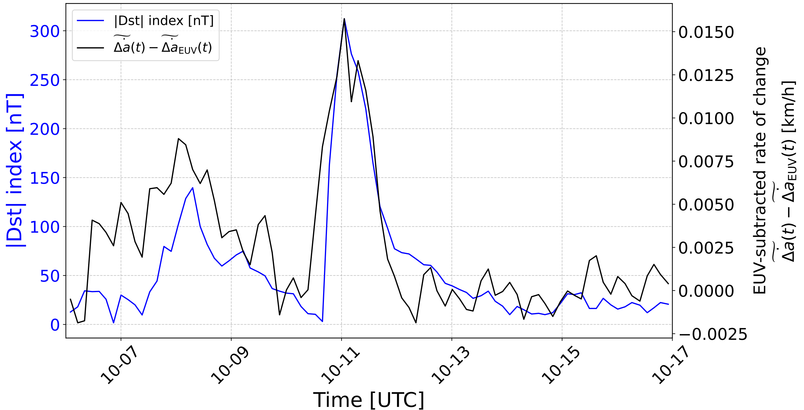
|Dst| index and EUV-subtracted rate of change for October 2024
