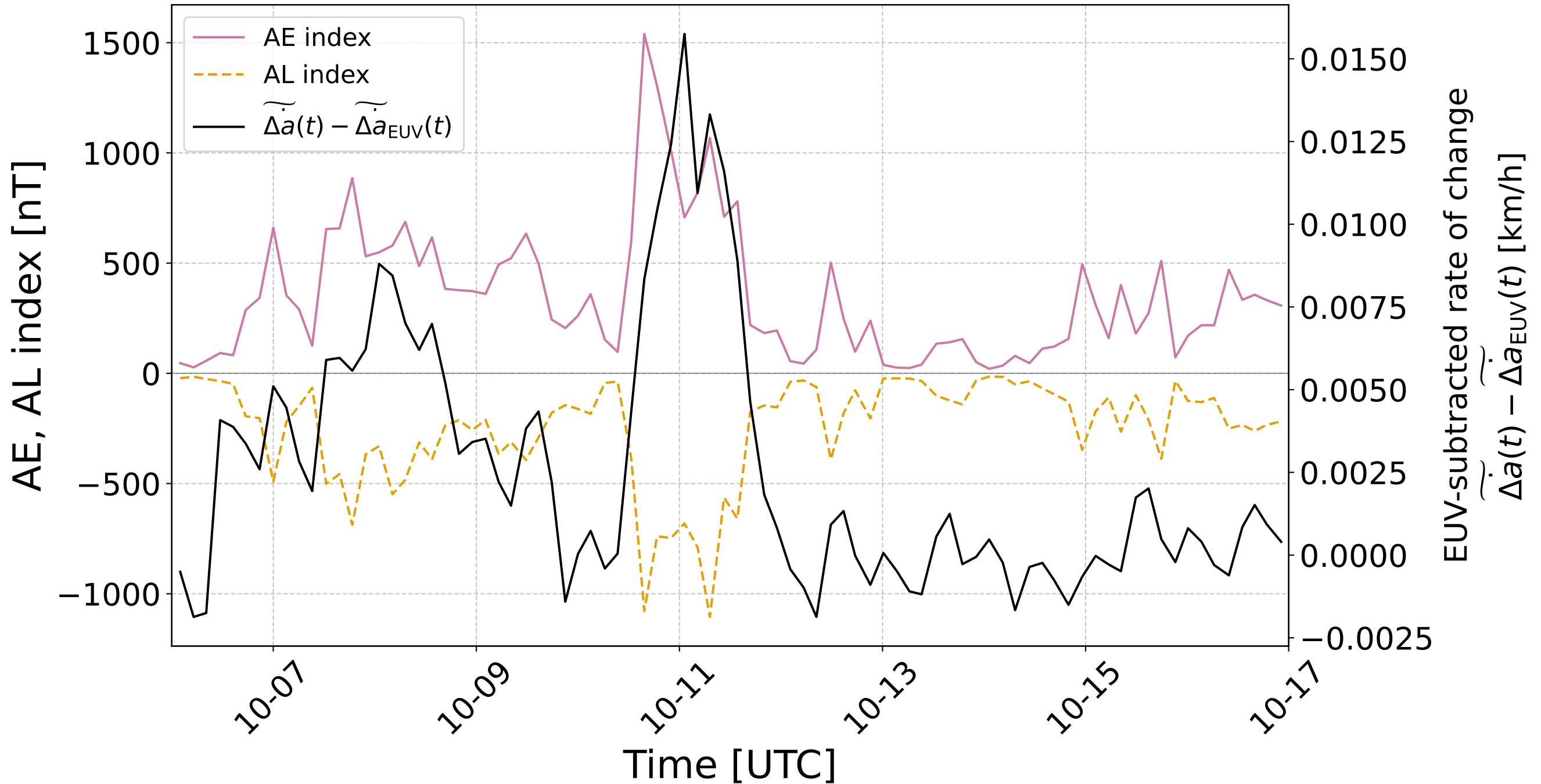
AE/AL indices and EUV-subtracted rate of change for October 2024
