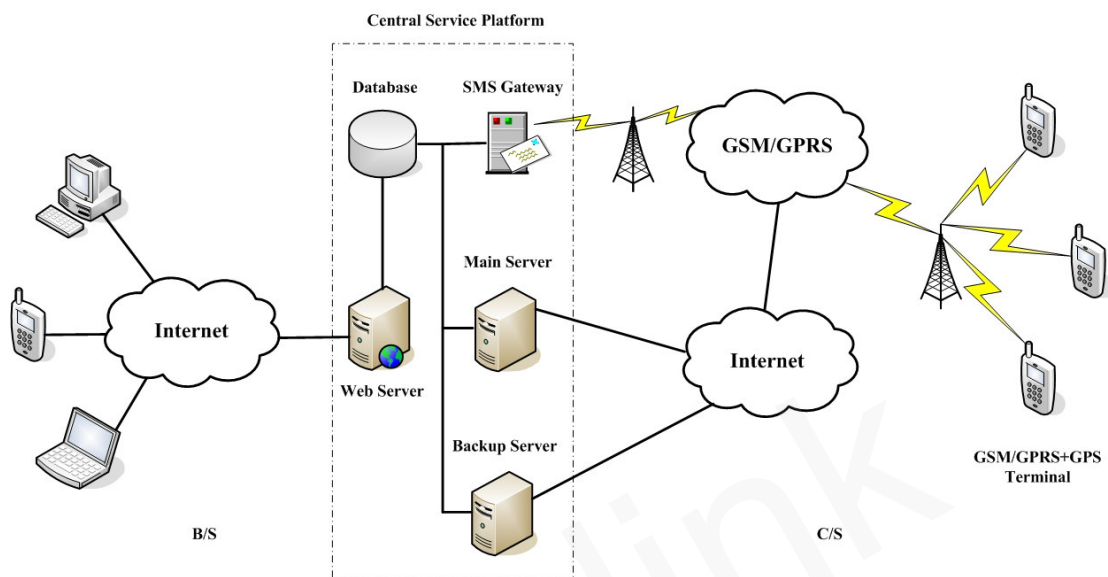
Figure 1: System architecture
