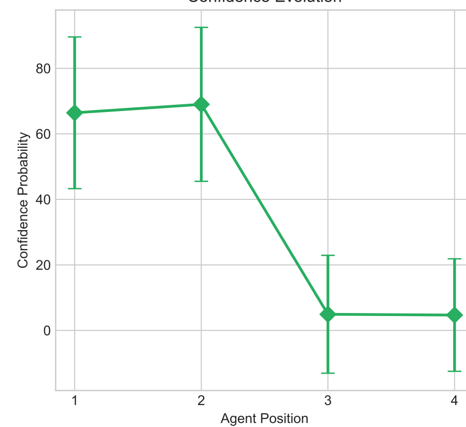
Confidence Evolution
