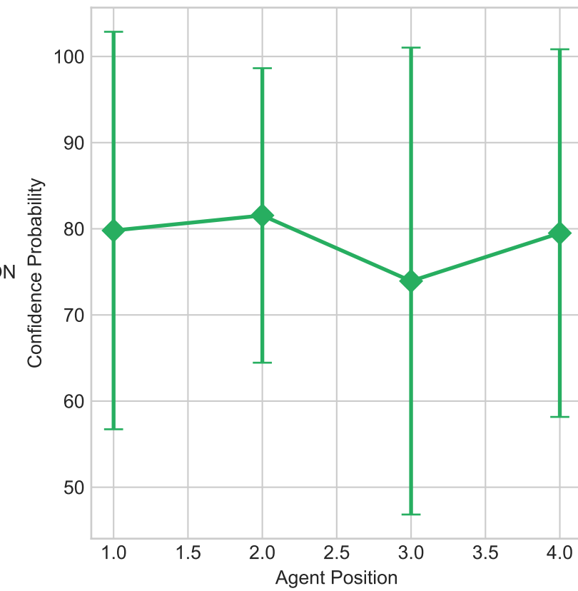
Confidence Evolution
