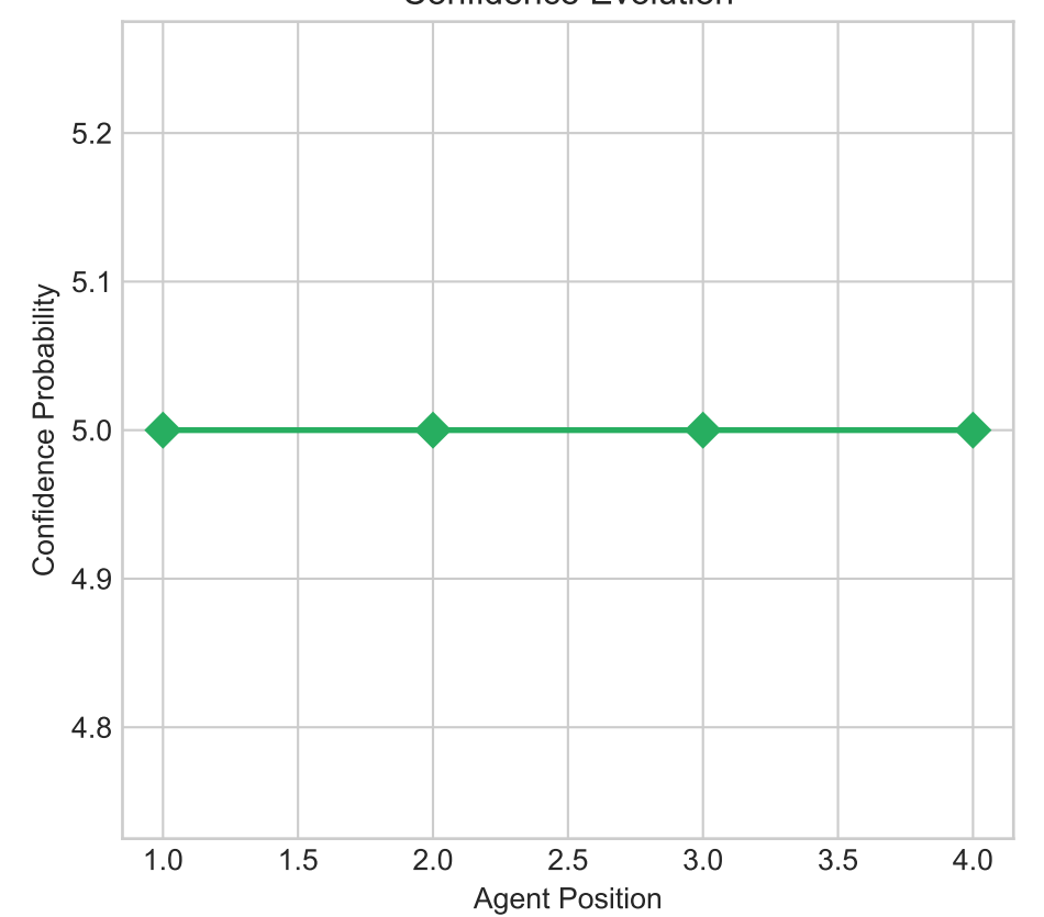
Confidence Evolution
