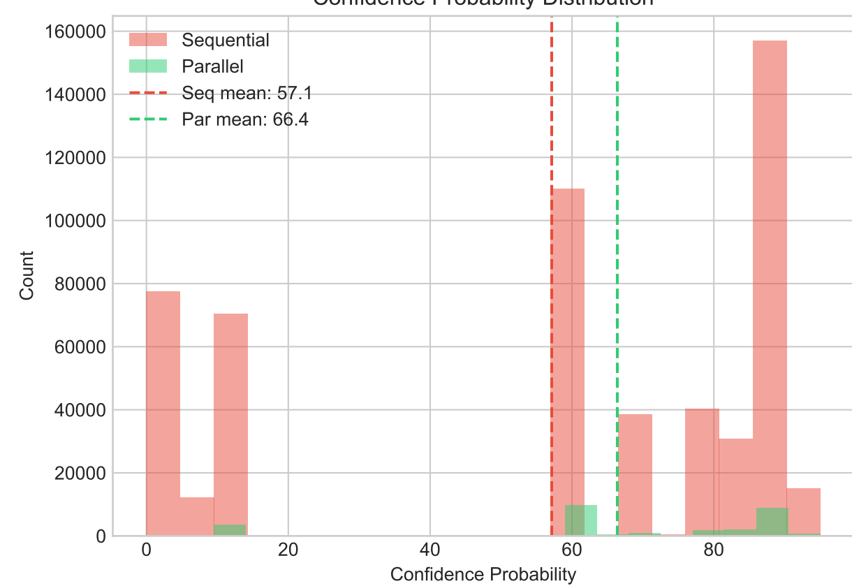
Confidence Probability Distribution
