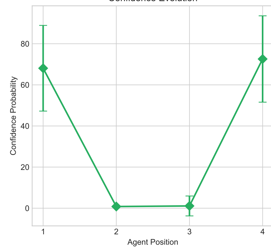
Confidence Evolution
