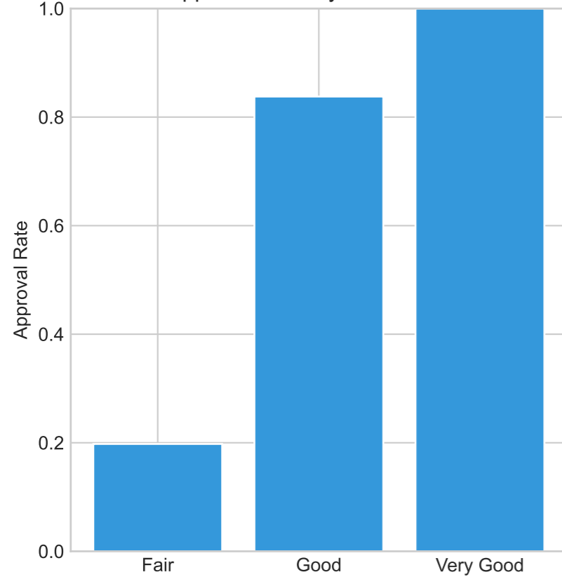
Approval Rate by Credit Score
