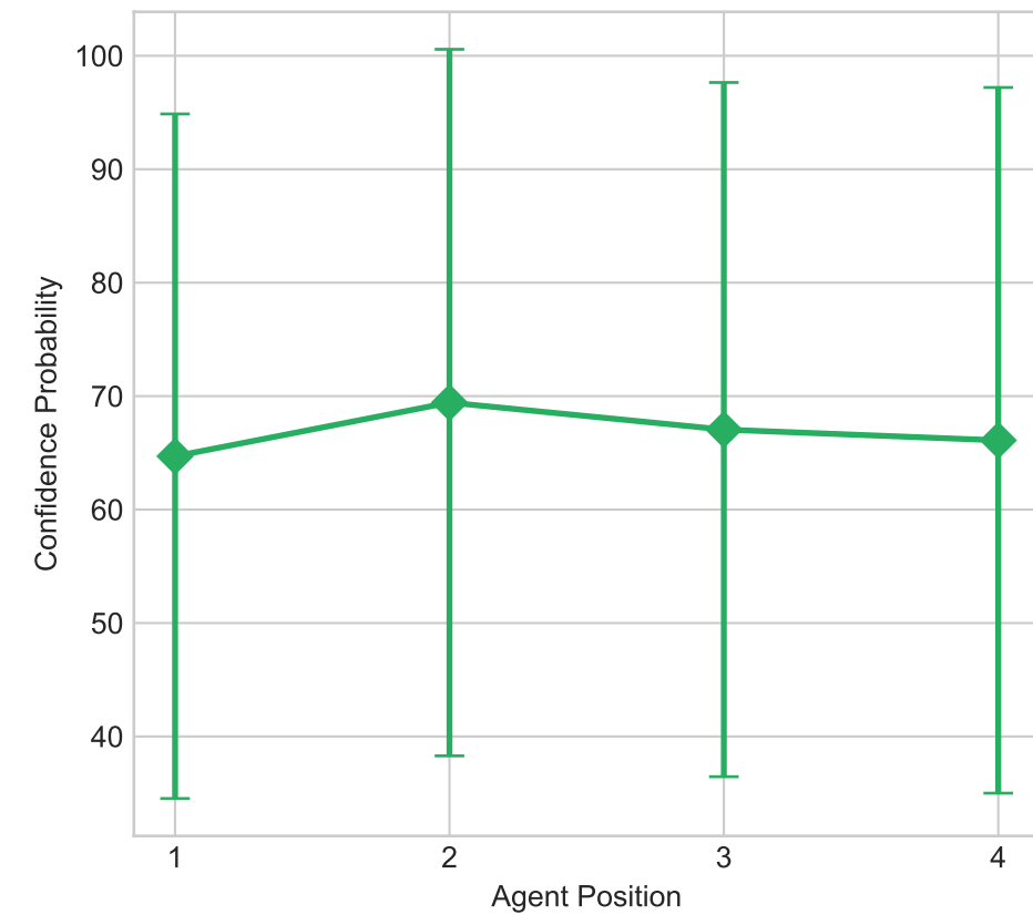
Confidence Evolution
