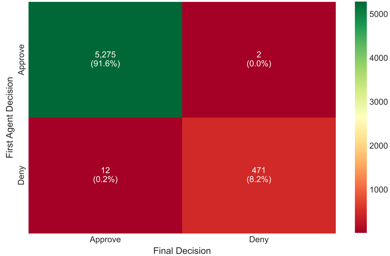
Decision Transition Counts
