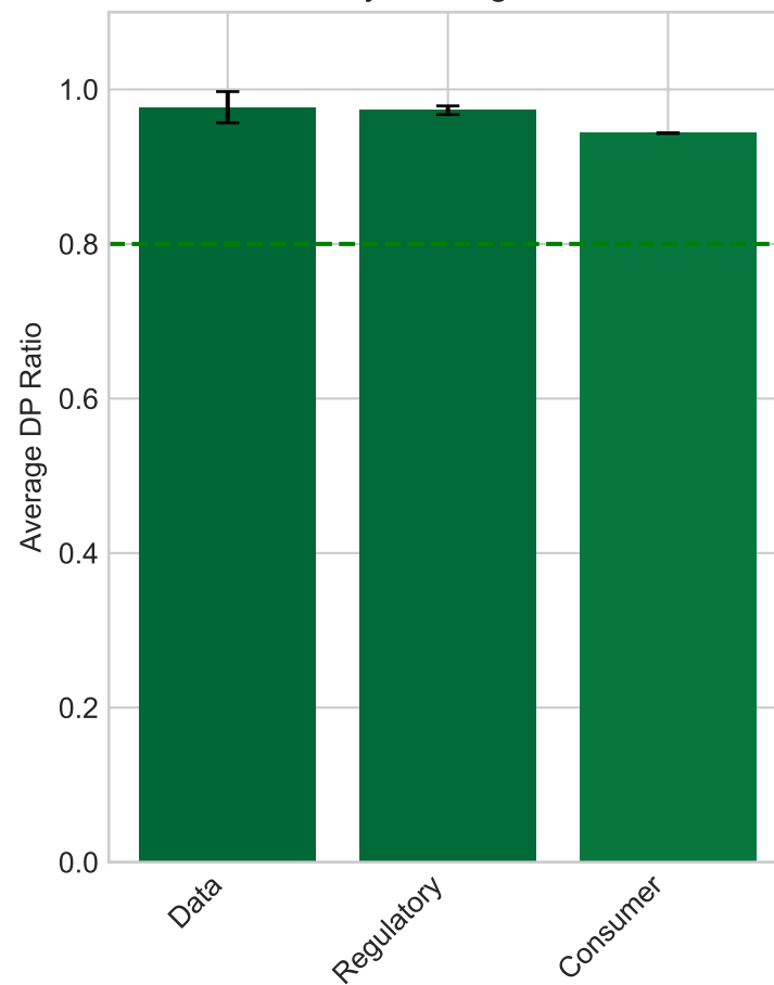
Fairness by First Agent in Chain
