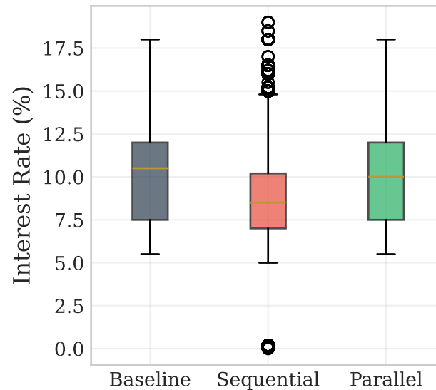
(b) Interest Rate Distribution
