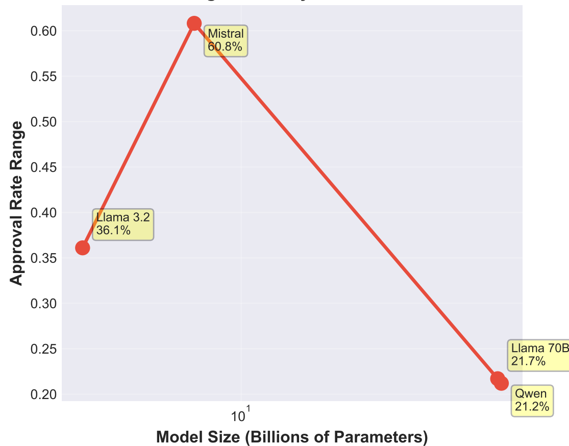
Ordering Sensitivity vs Model Scale
