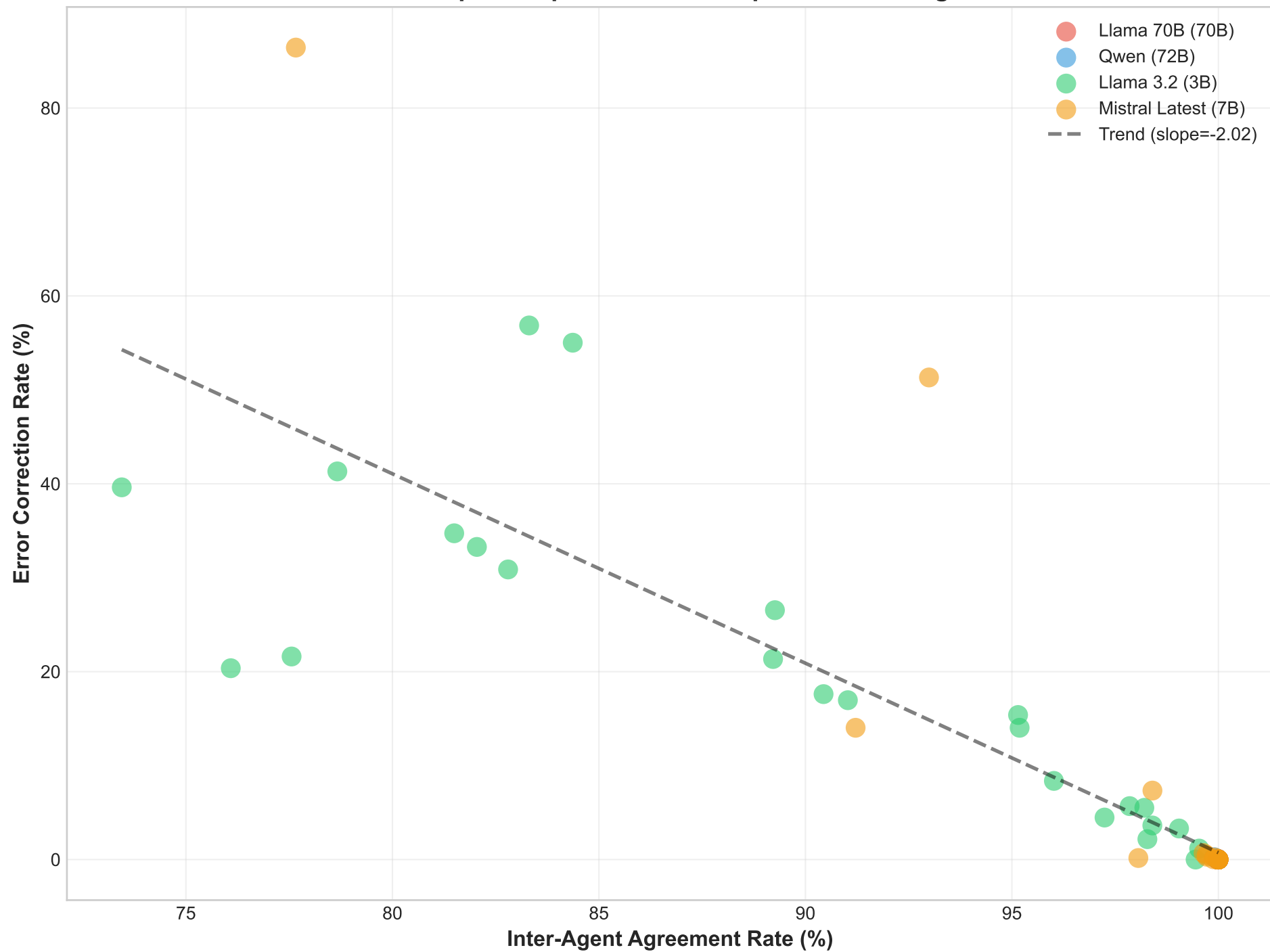
The Scale Paradox: High Agreement Low Error Correction Each point represents one sequential ordering
