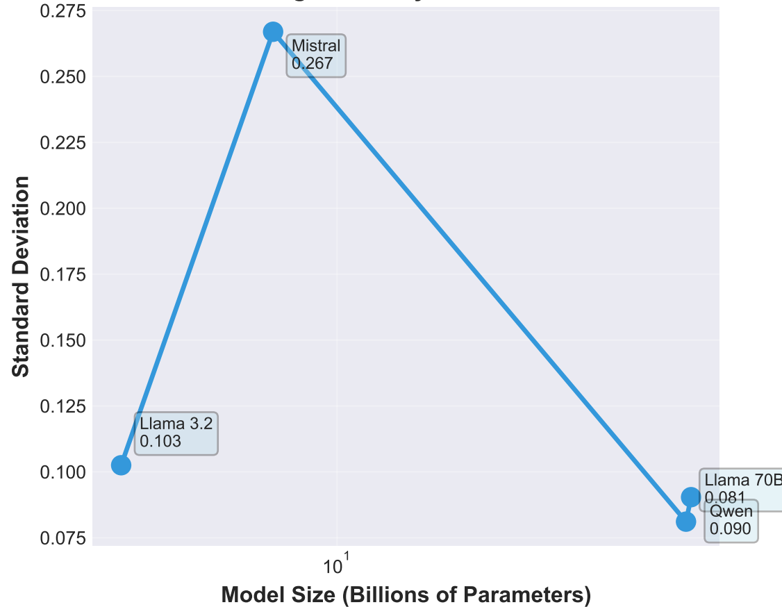
Ordering Variability vs Model Scale
