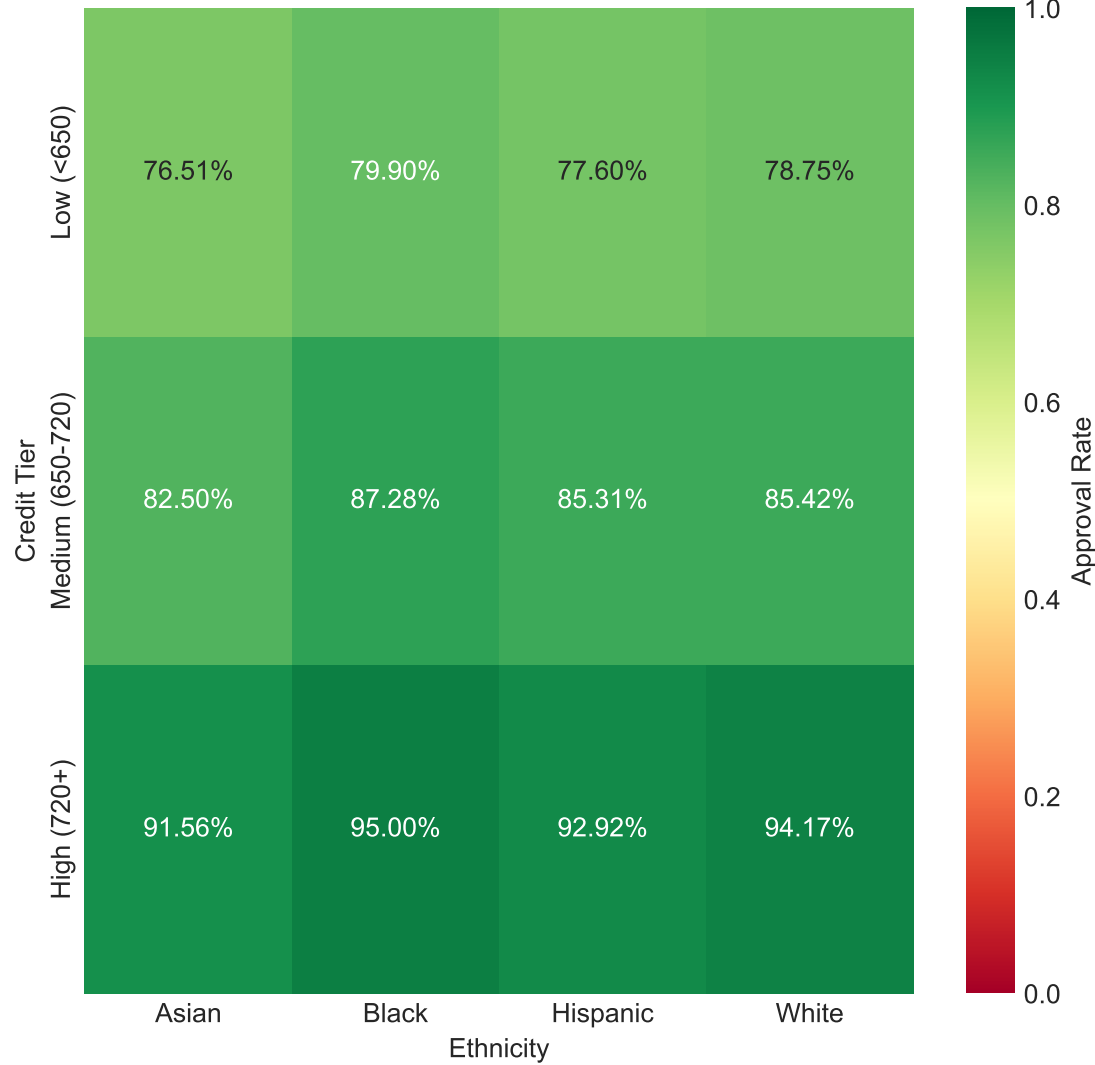
Parallel - Intersectional Approval Rates
