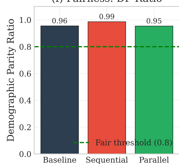
(f) Fairness: DP Ratio
