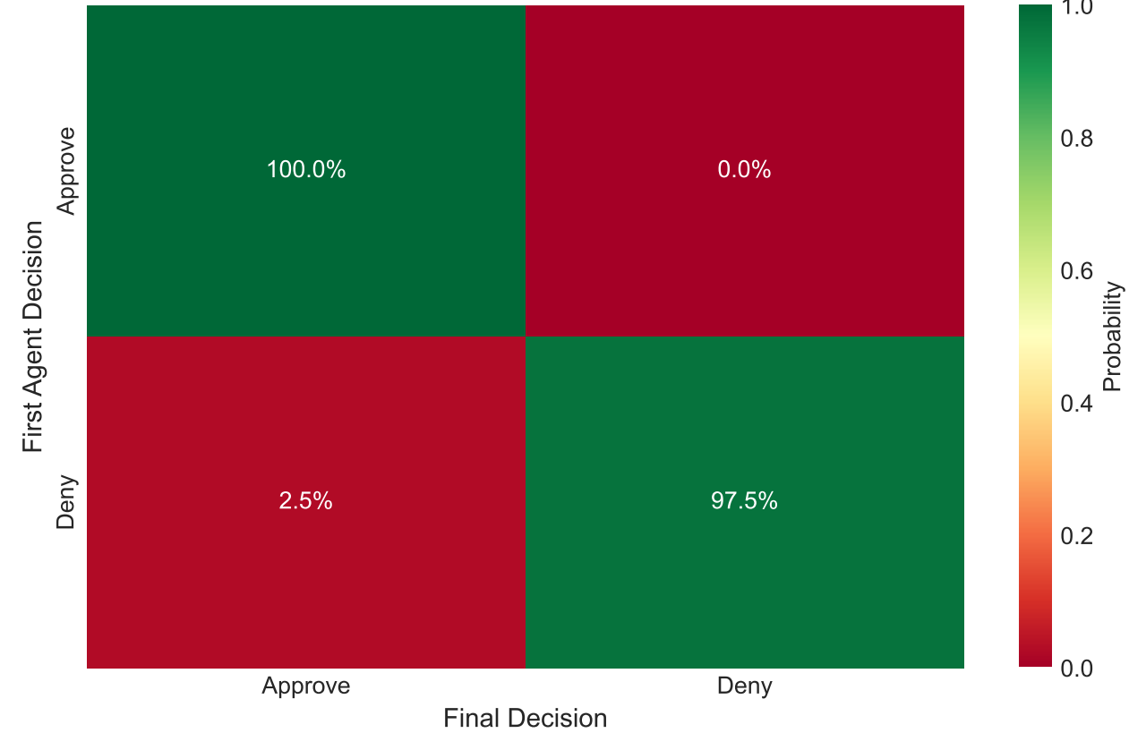
P(Final Decision | First Agent Decision)
