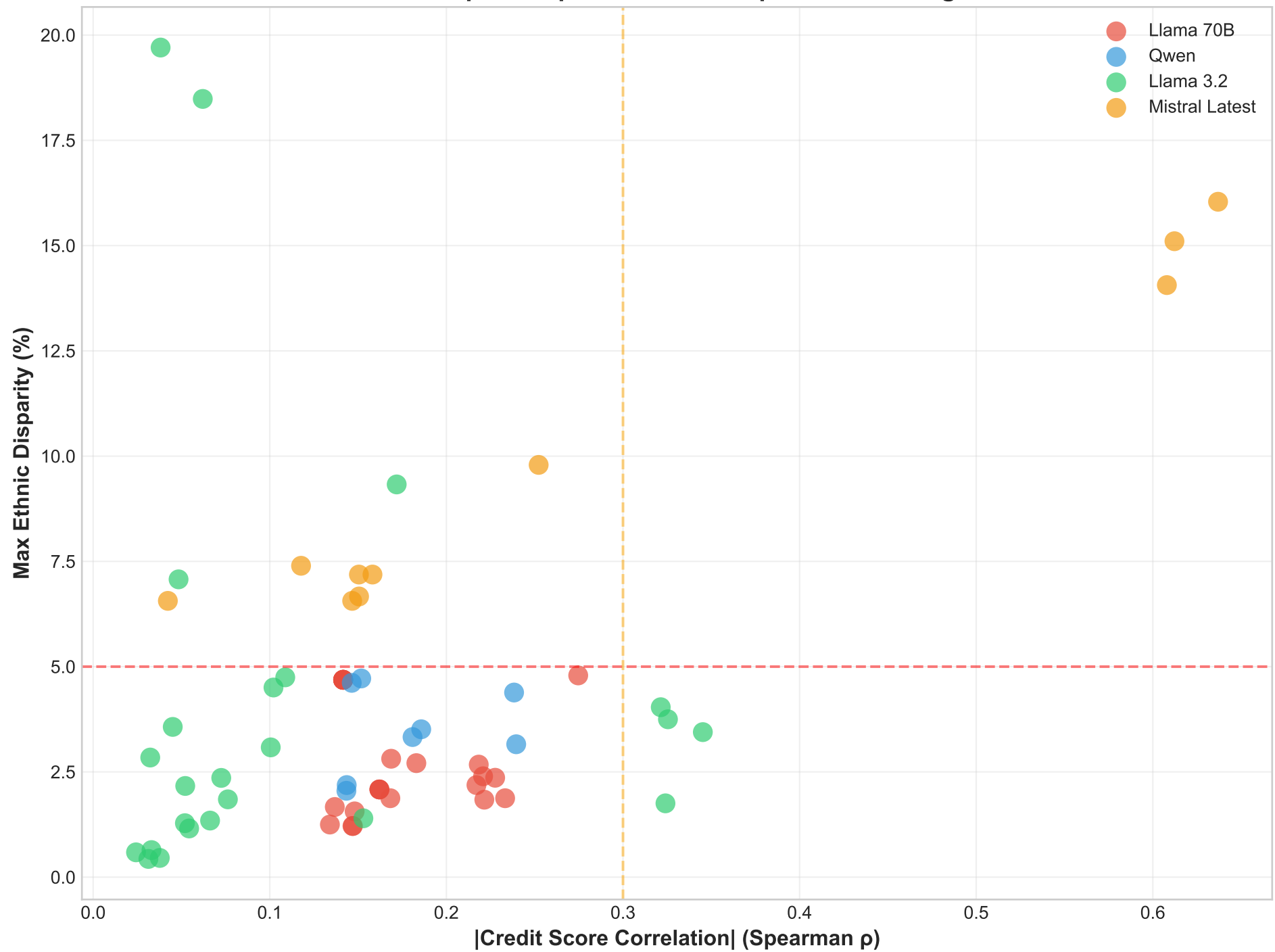
Functional Collapse: Demographic Parity vs Credit Score Correlation Each point represents one sequential ordering
