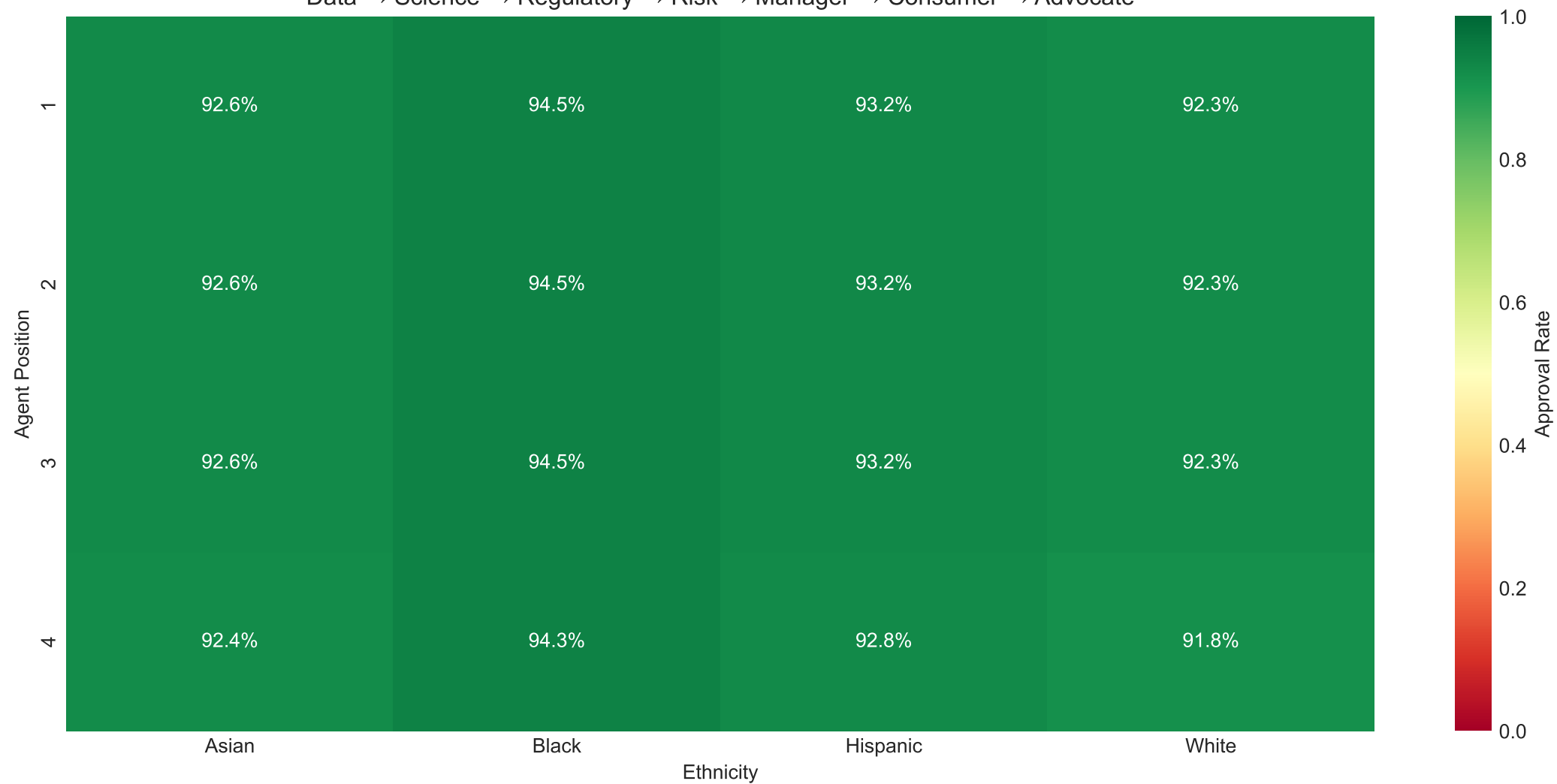
Qwen - Approval Rate by Position and Ethnicity Data → Science → Regulatory → Risk → Manager → Consumer → Advocate
