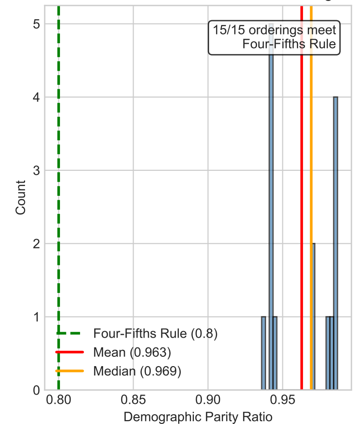
Distribution of Fairness Across Orderings
