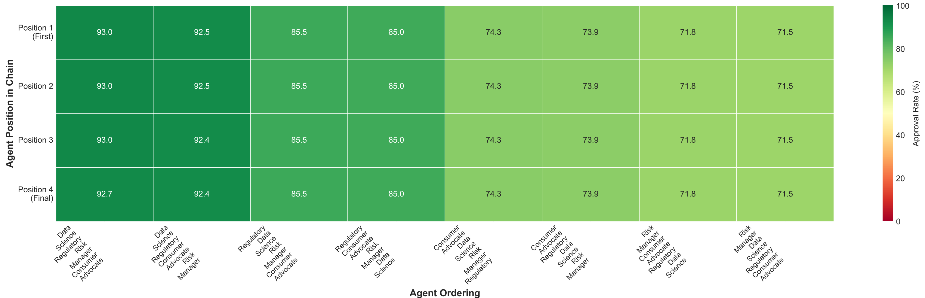
Qwen Model: Approval Rates by Agent Position Across All Orderings (80.7% = Overall Average)
