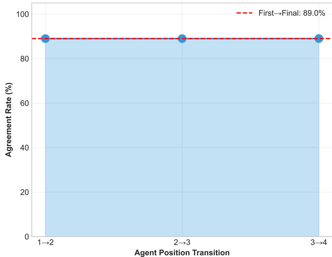
Qwen - Information Cascade
