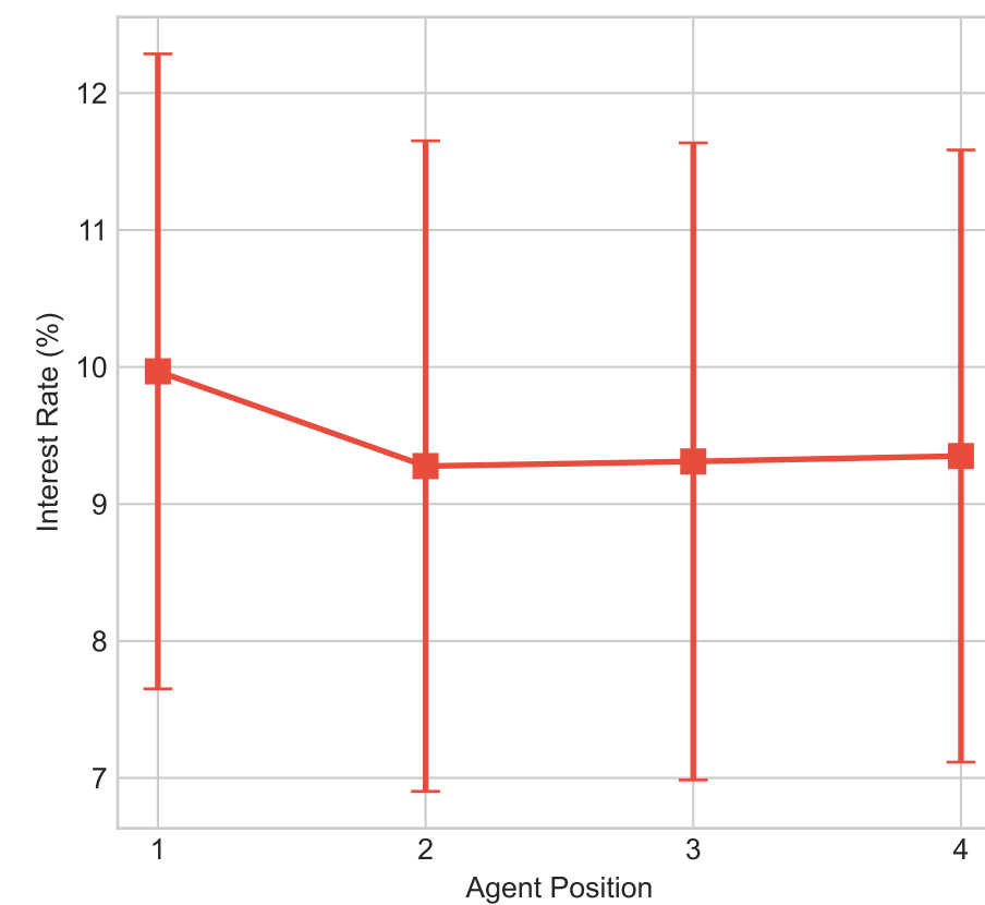
Confidence Evolution
