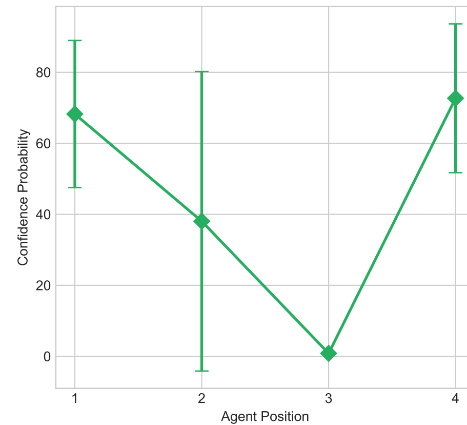
Confidence Evolution
