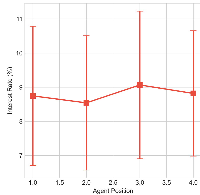
Confidence Evolution
