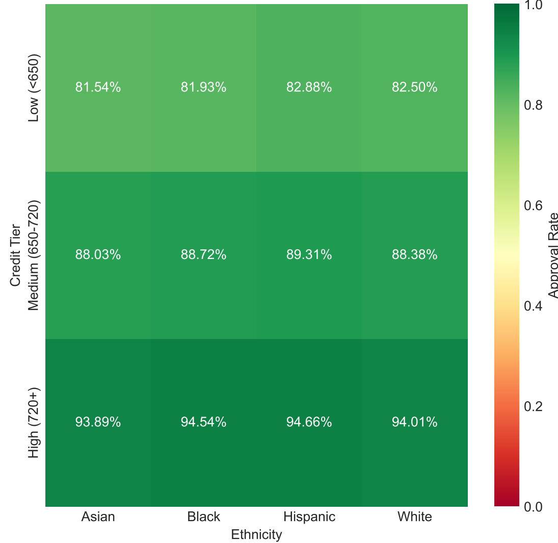
Sequential - Intersectional Approval Rates
