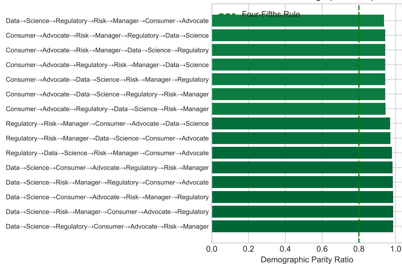
Fairness by First Agent in Chain
