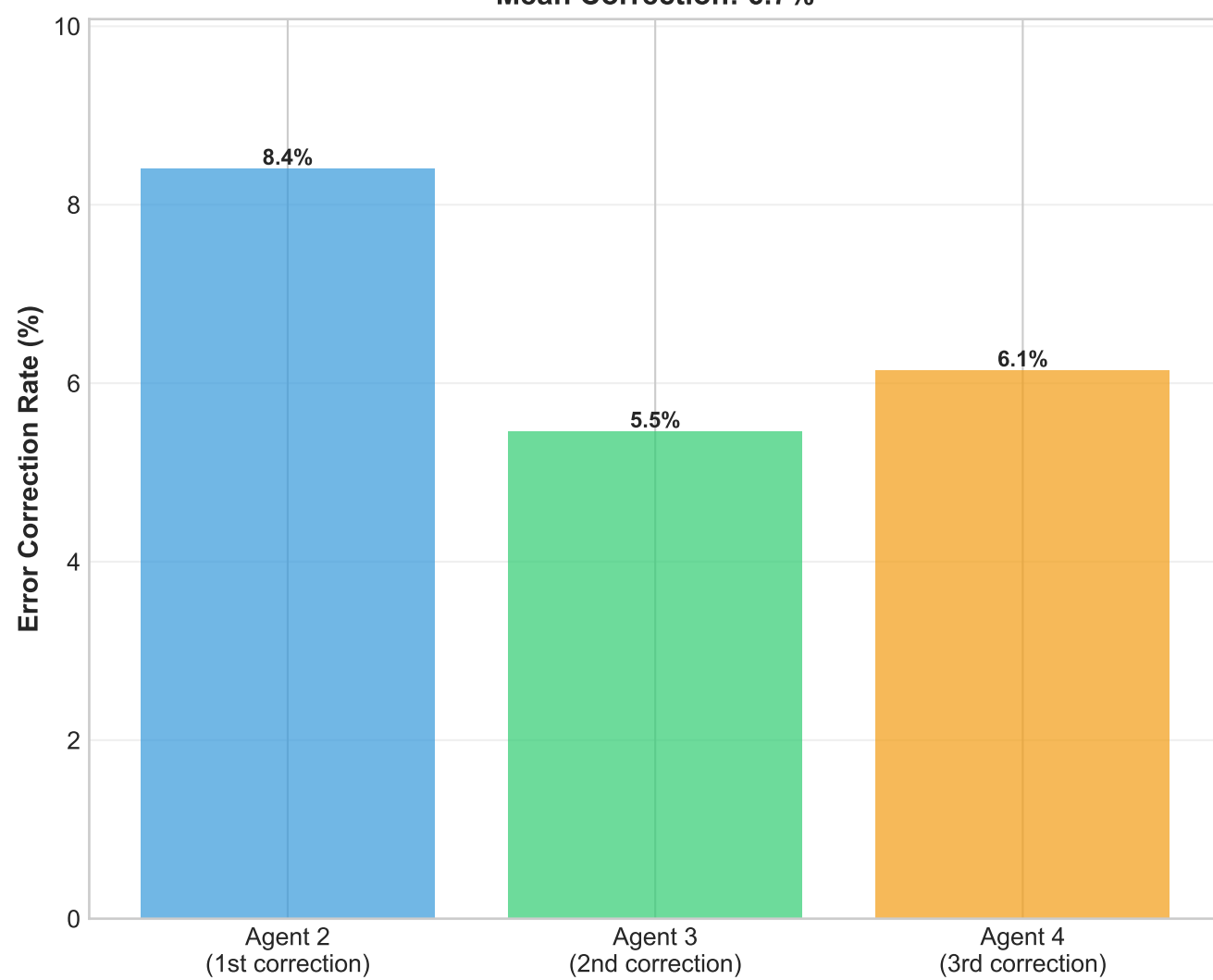
Llama 3.2 (3B Parameters) Mean Correction: 6.7%
