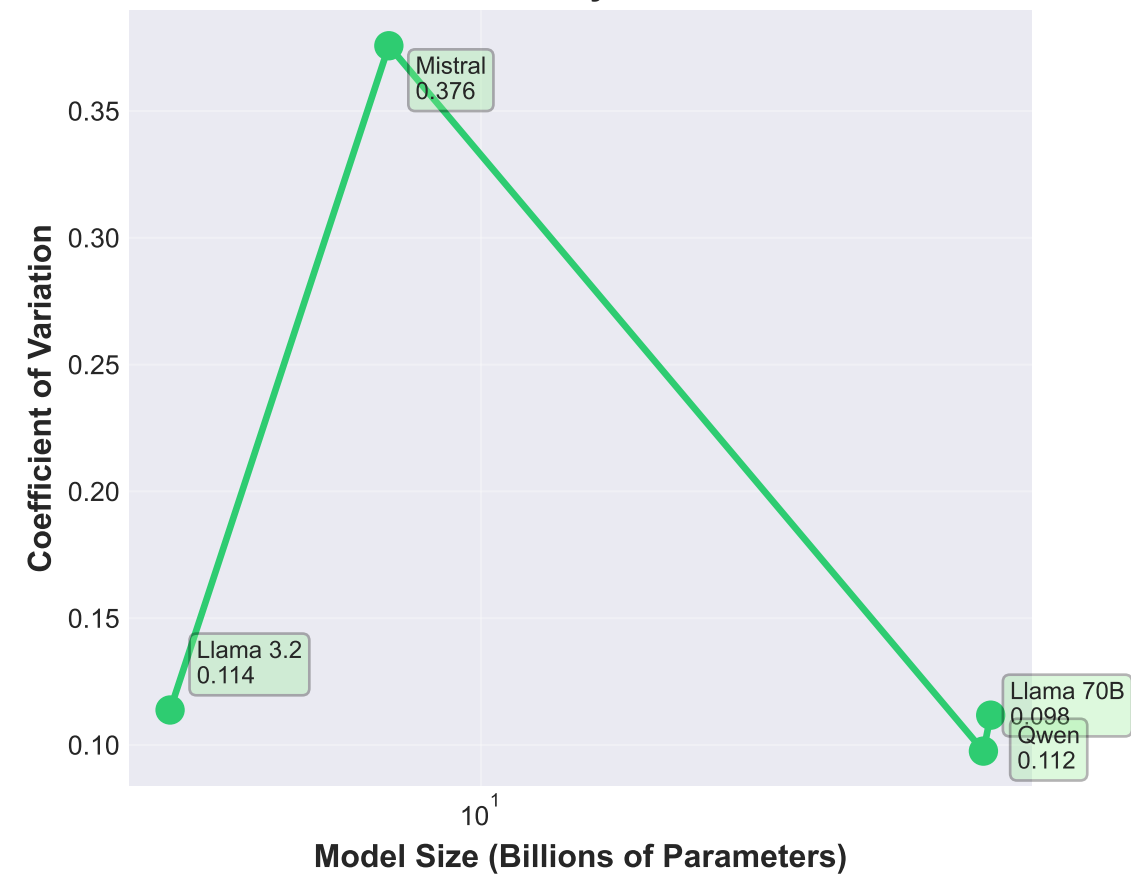
Relative Sensitivity vs Model Scale
