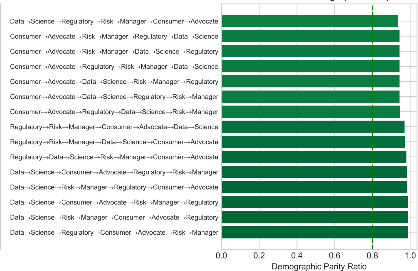
Distribution of Fairness Across Orderings
