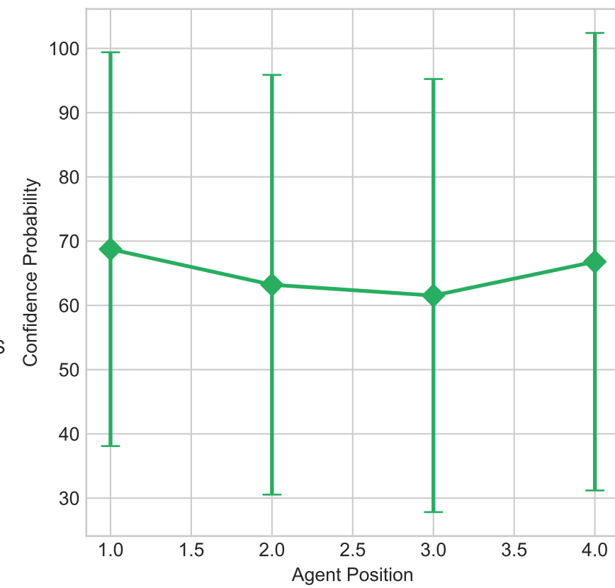
Confidence Evolution
