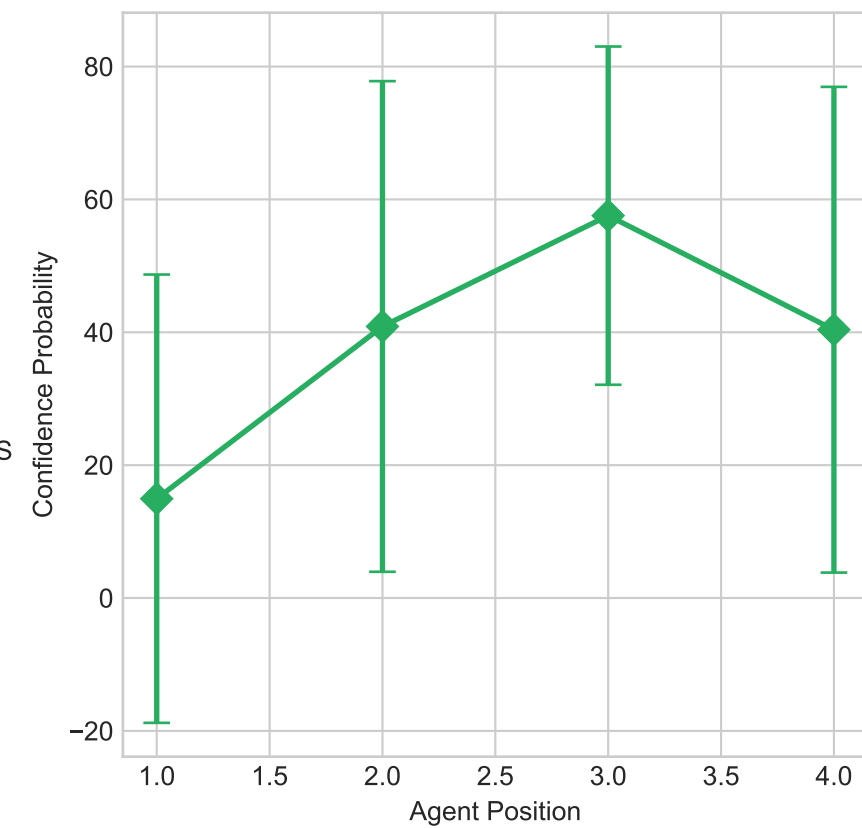
Confidence Evolution
