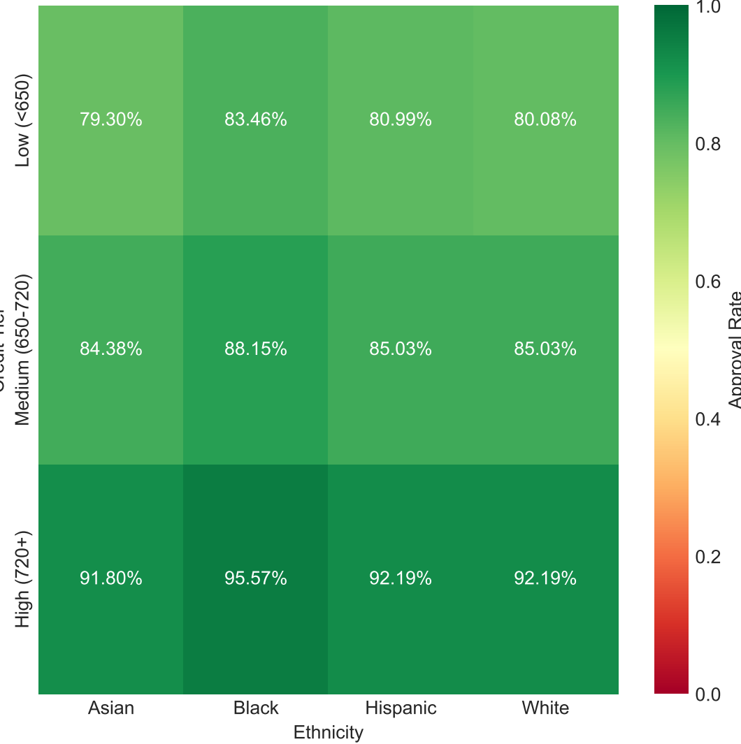
Baseline - Intersectional Approval Rates
