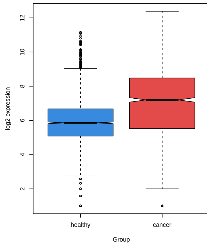
Top miRNA: hsa-miR-6131 log2FC = 2.79
