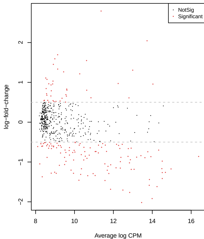
MA plot (red = significant, flat cloud = good)
