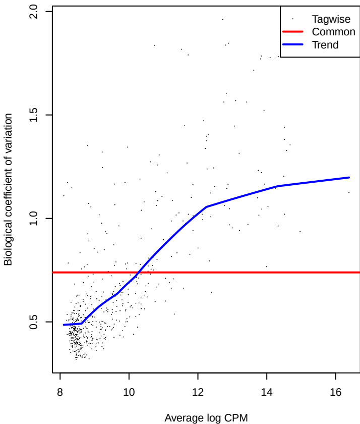
Biological Coefficient of Variation (tagwise should follow trend)
