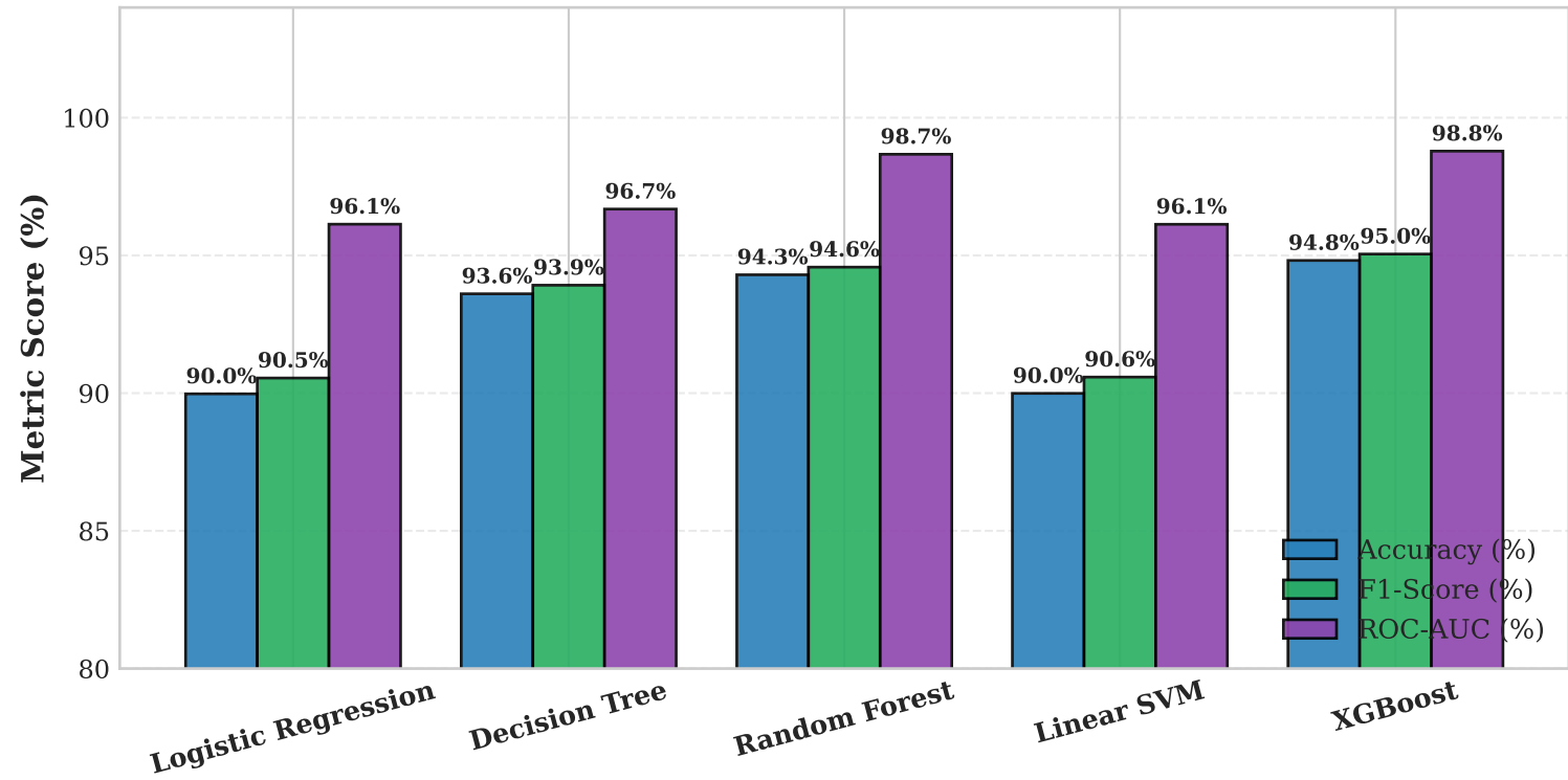
Comparative Performance Across Evaluated Machine Learning Models
