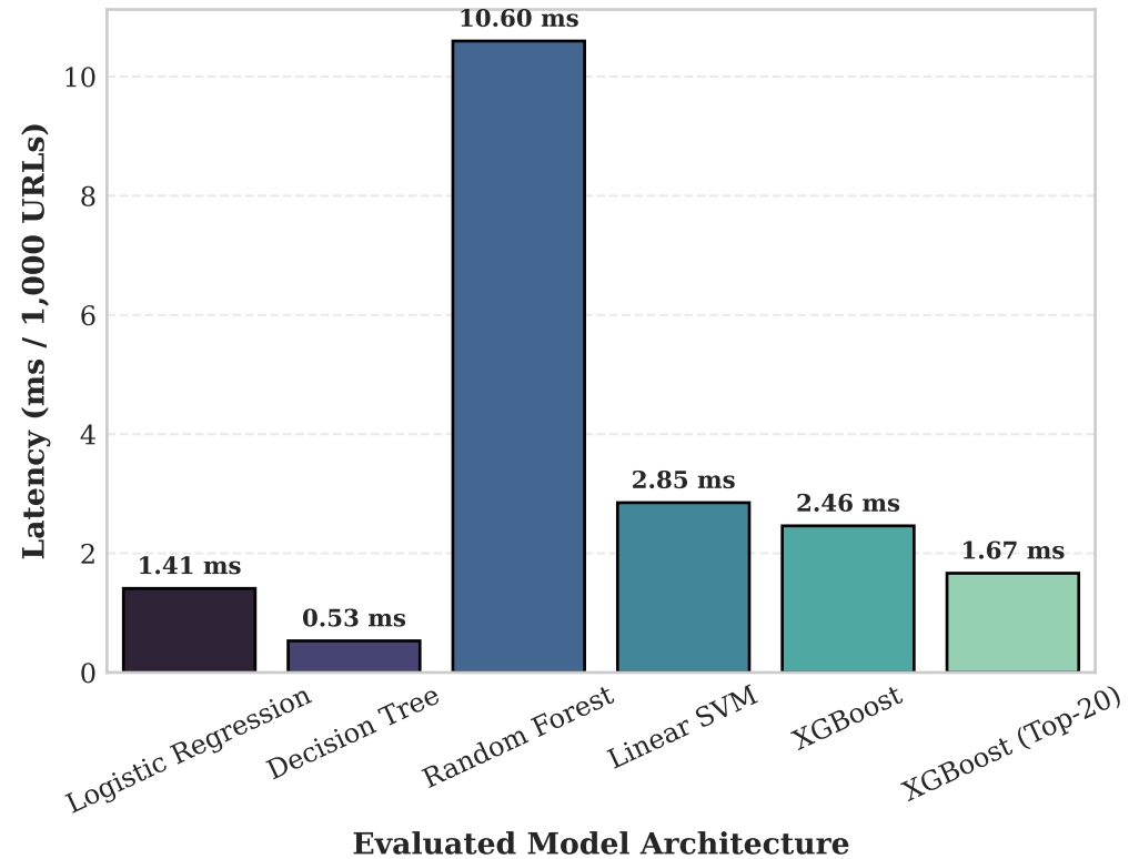
Inference Latency (ms / 1k Queries)
