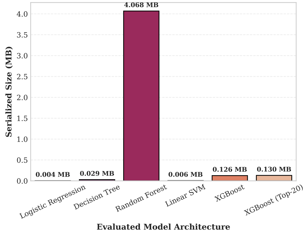
Serialized Model Storage Footprint (MB)
