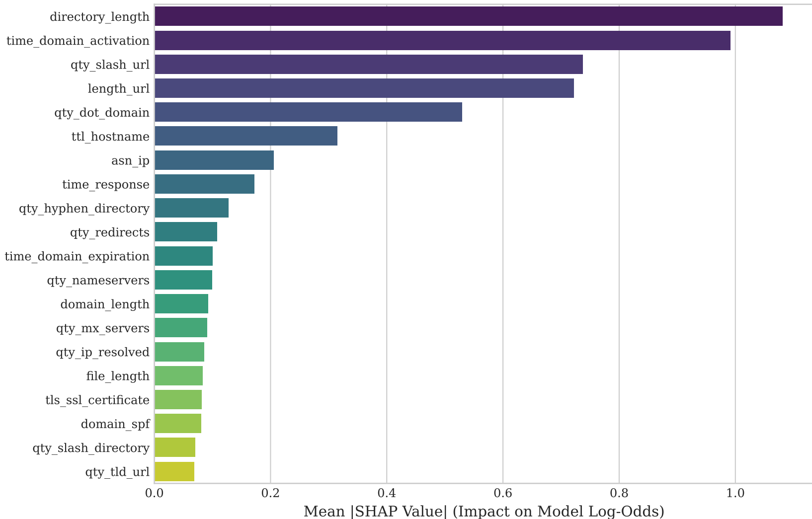
Top 20 Most Influential Features (Mean |SHAP Value| on Training Set)
