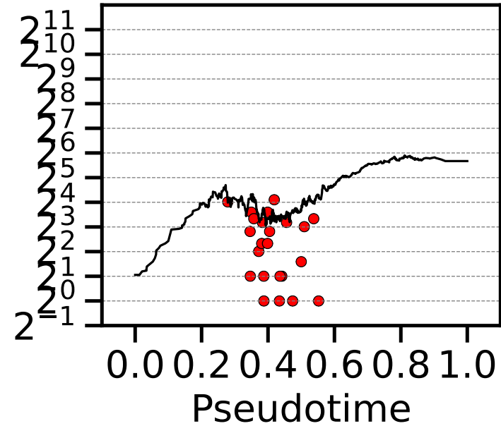
HBD
