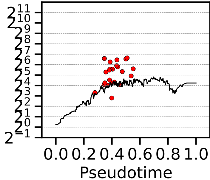
HBG2
