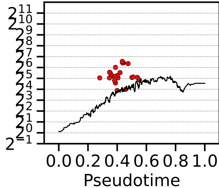
HBG1
