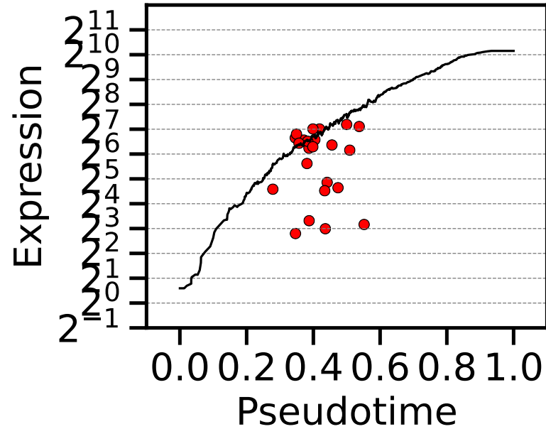
HBB
