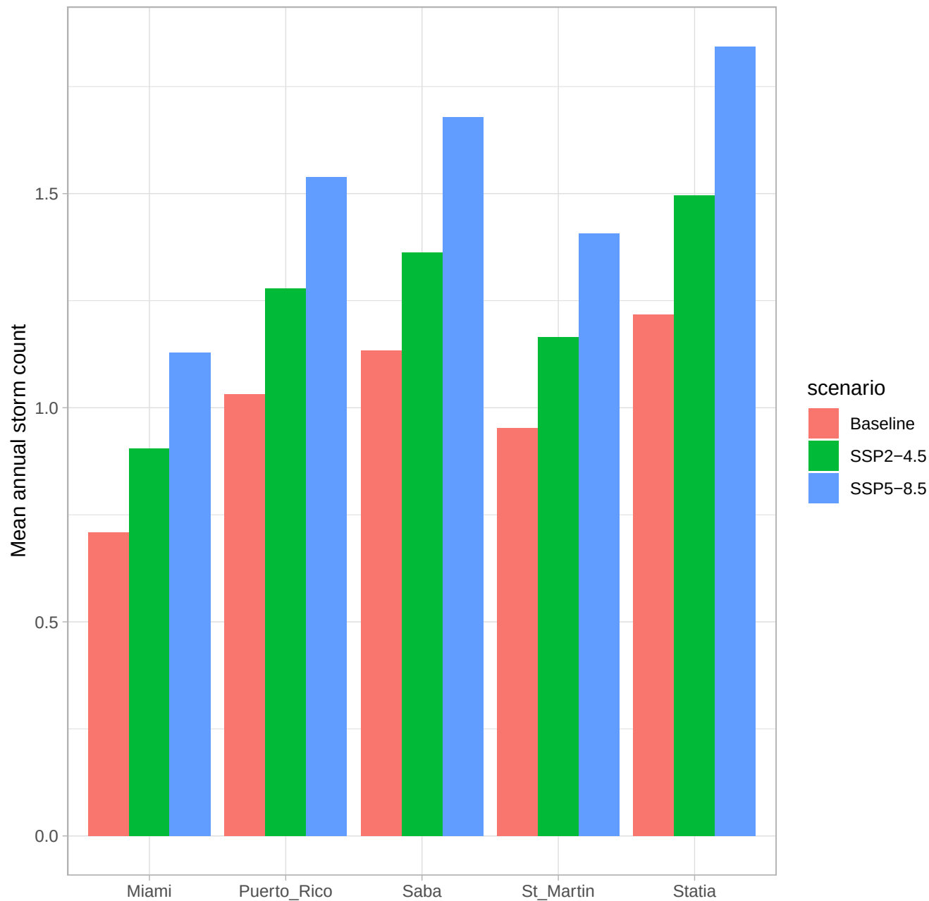
Simulated annual storm activity by scenario
