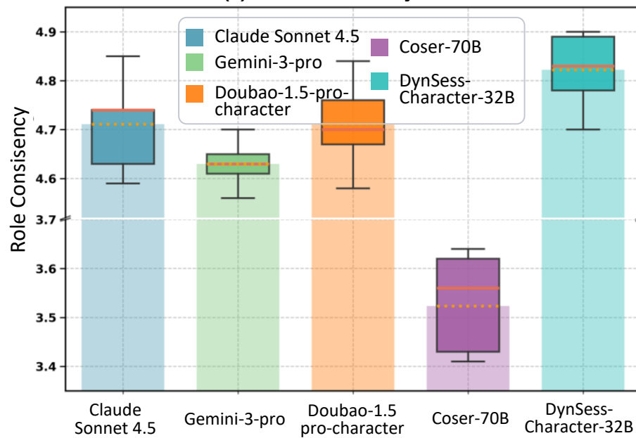
(c). Role Consistency.
