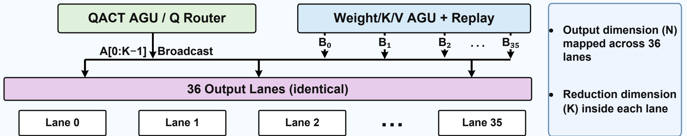
(a) Standard spatial/linear mode (conventional GEMM-style mapping)
