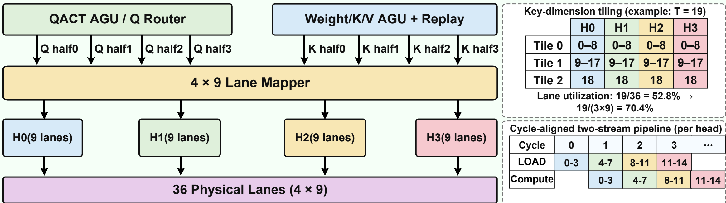
(b) Temporal QK with output-axis adaptation (4-head packing with overlapped Q/K delivery)
