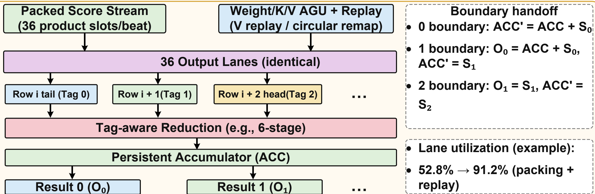
(c) Temporal PV with reduction-axis adaptation (V replay + segmented reduction)
