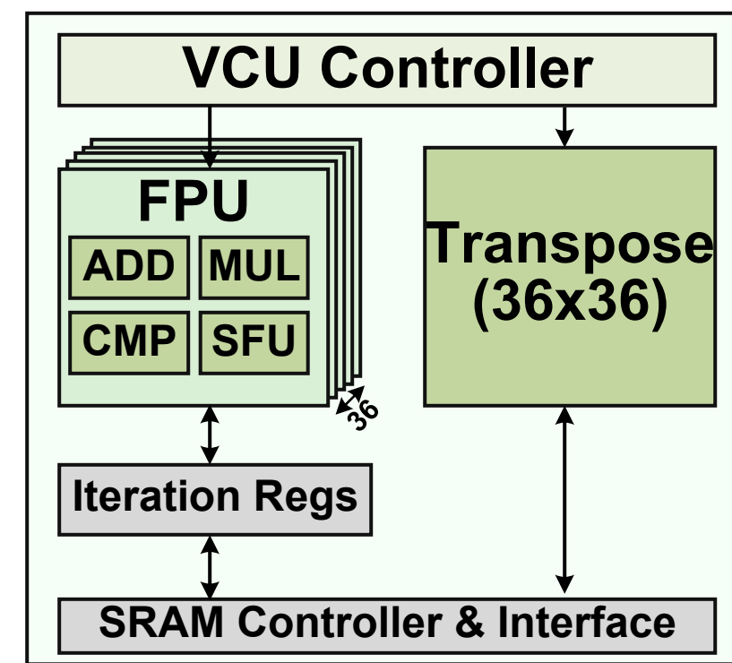
(c) The structure of the VCU
