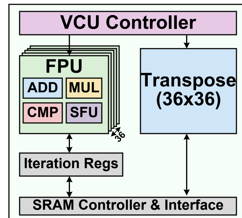
(c) The structure of the VCU
