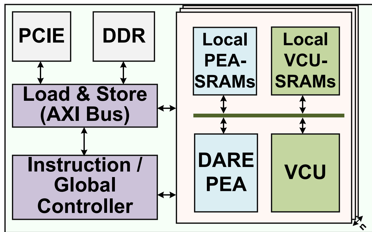
(a) Top-level accelerator architecture
