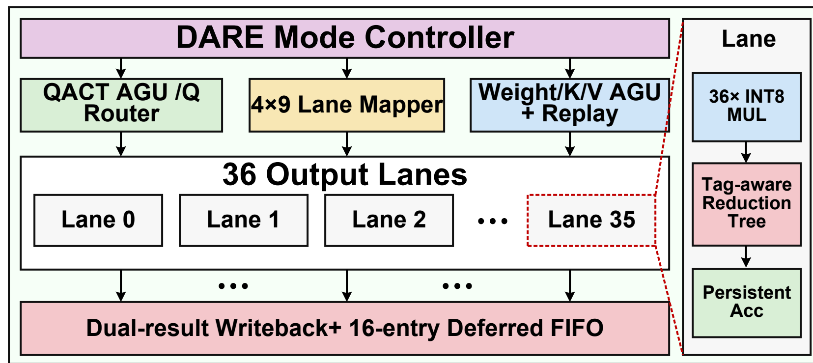
(b) The microarchitecture of the DARE processing engine (PEA)
