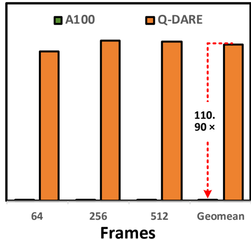
(b) Energy Efficiency (steps/s/kW)
