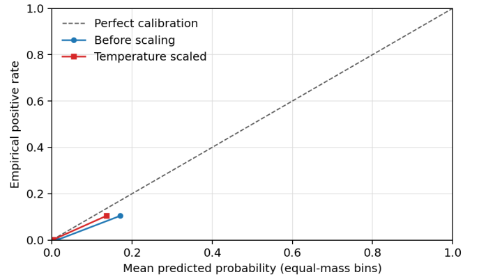
Fig. 3. Reliability diagram on the combined validation split. Temperature scaling reduces aggregate error. Equal-mass bins expose sparsely populated confidence regions.
